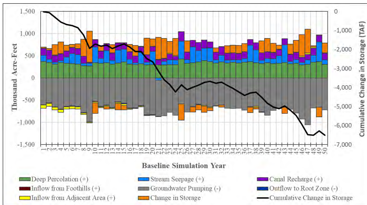
Figure 2-127: Groundwater Budget - MercedWRM Climate Change Scenario
