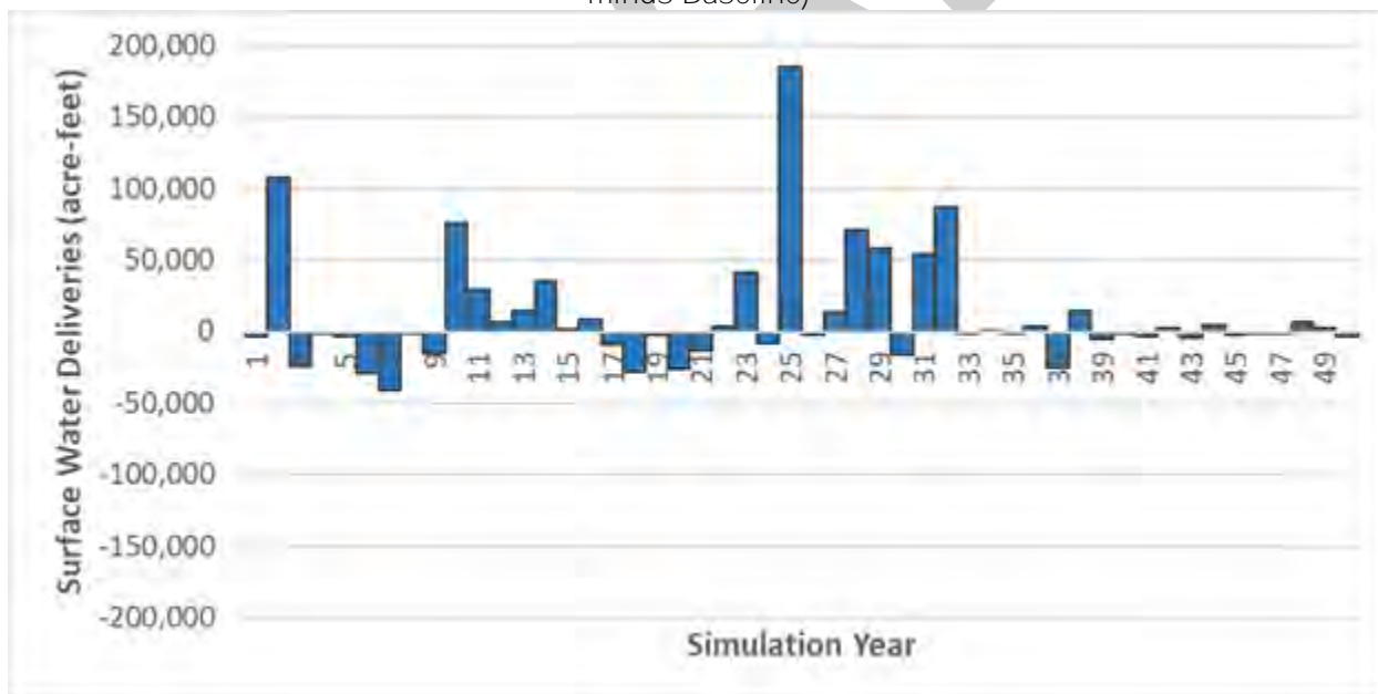
Figure 2-124: Simulated Changes in Surface Water Supplies due to Climate Change (Scenario minus Baseline)
