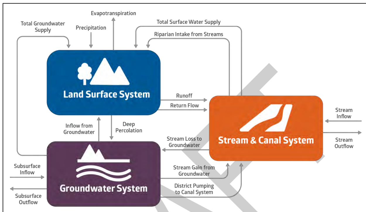
Figure 2-89: Generalized Water Budget Diagram
