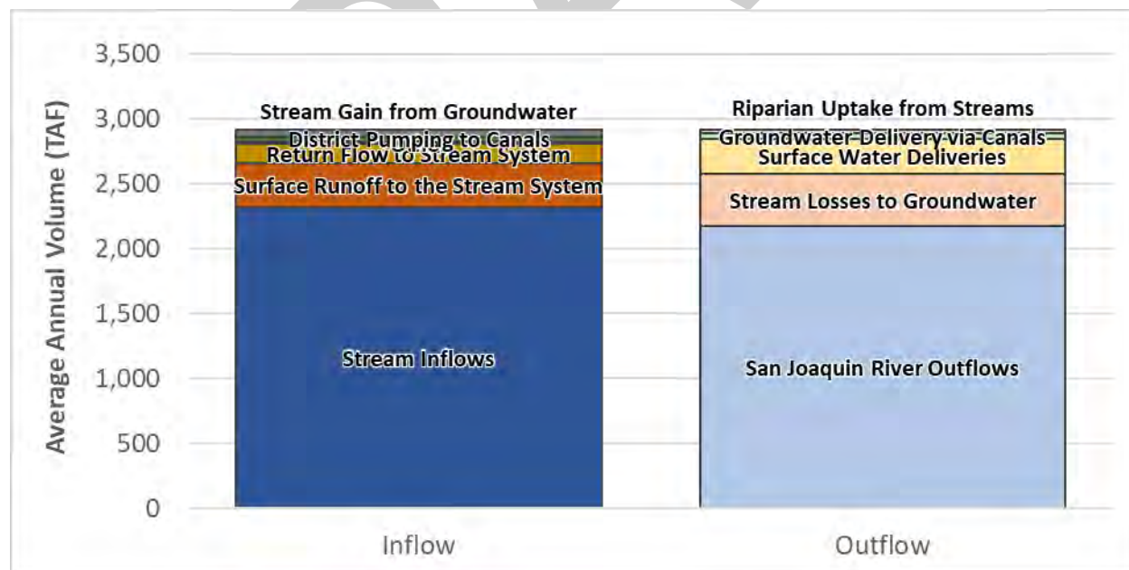
Figure 2-101: Projected Conditions Average Annual Water Budget – Stream and Canal Systems, Merced Subbasin
