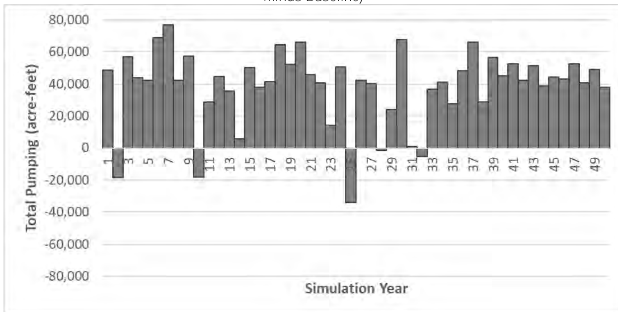
Figure 2-125: Simulated Changes in Groundwater Production due to Climate Change (Scenario minus Baseline)
