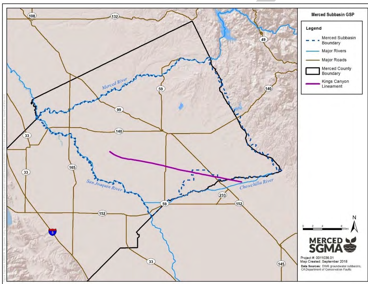
Figure 2-26: Fault Map
