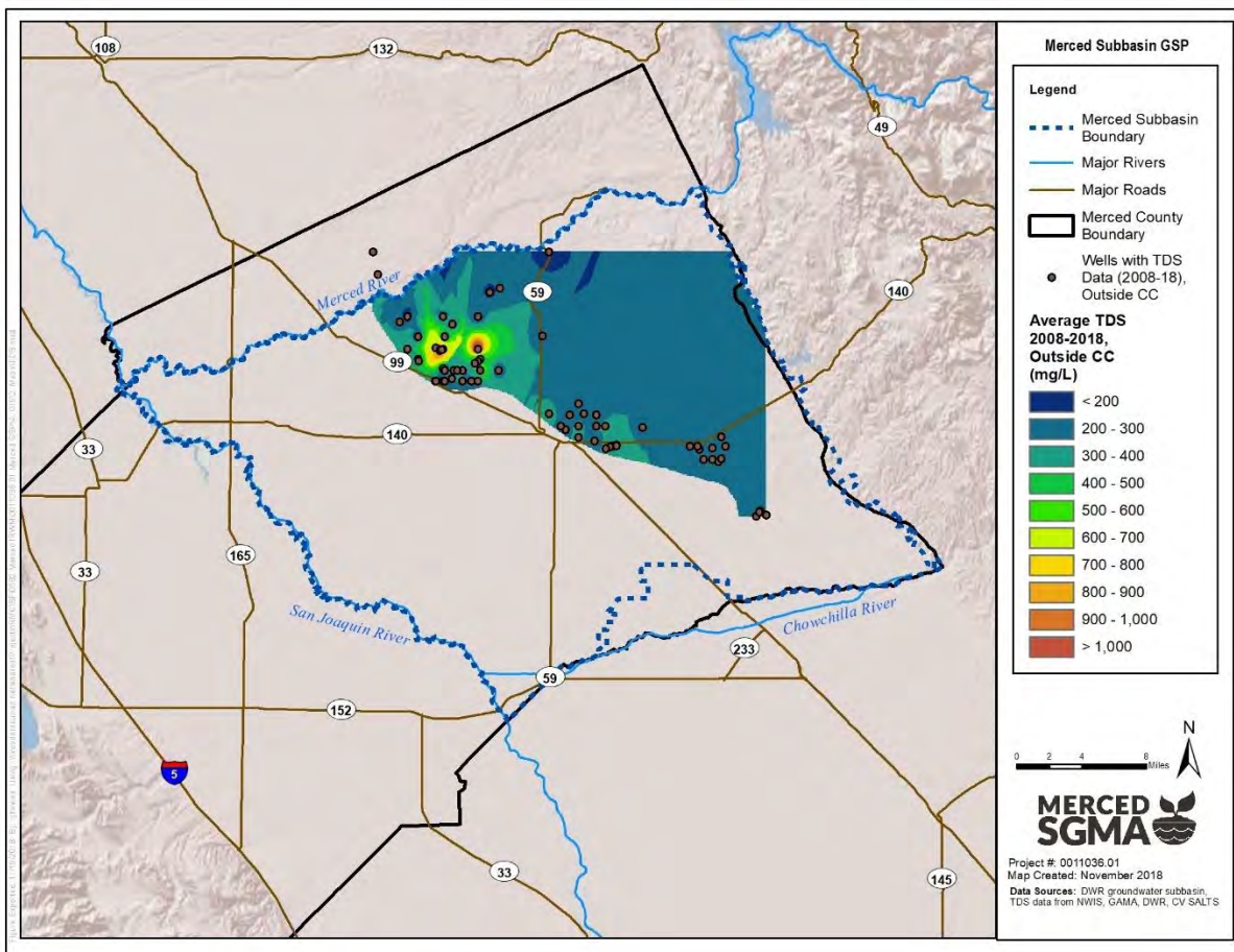
Figure 2-65: Average TDS Concentration 2008-2018, Outside Corcoran Clay
