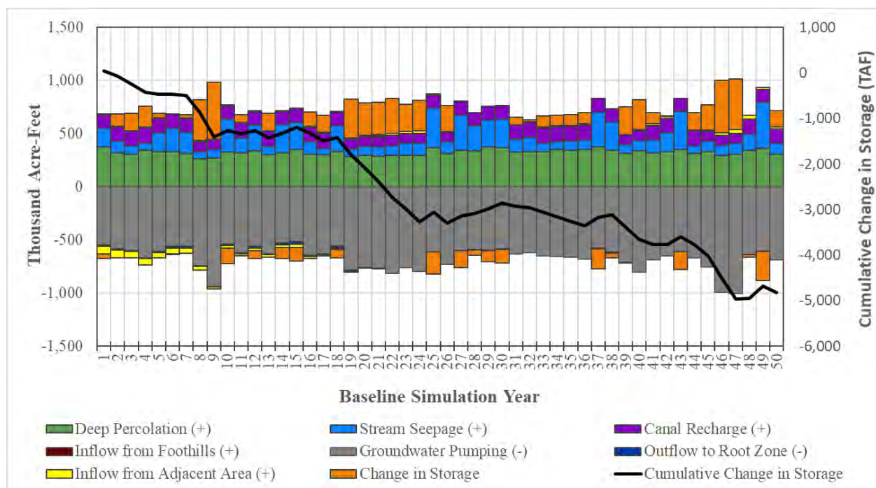
Figure 2-105: Projected Conditions Annual Water Budget – Groundwater System, Merced Subbasin
