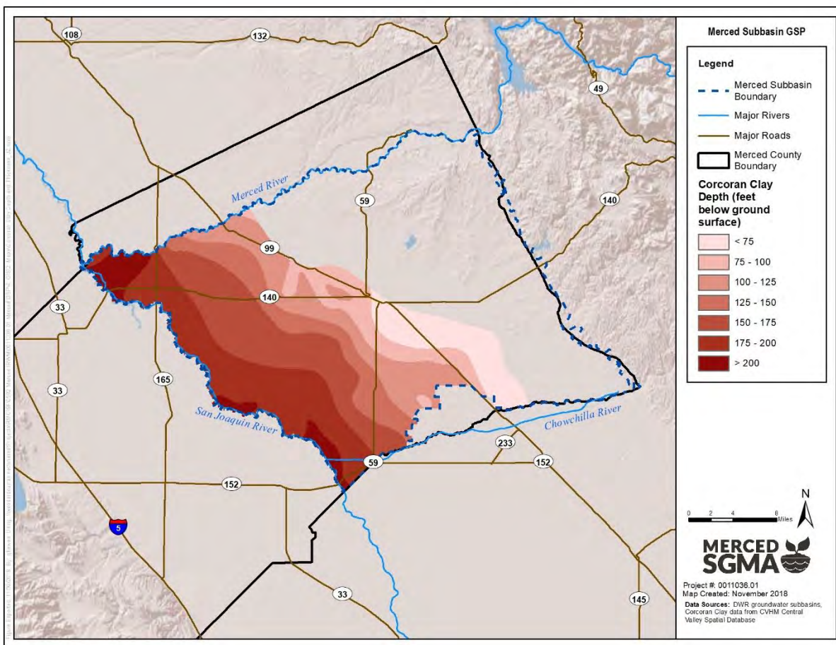
Figure 2-37: Corcoran Clay Depth Below Ground Surface
