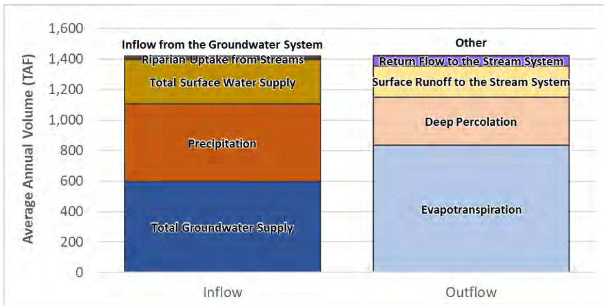
Figure 2-98: Current Conditions Annual Water Budget – Land Surface System, Merced Subbasin
