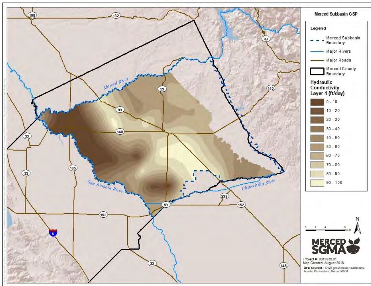
Figure 2-30: Hydraulic Conductivity – Confined Aquifer (MercedWRM Layer 4)
