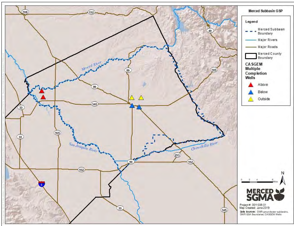
Figure 2-50: CASGEM Multiple Completion Wells
