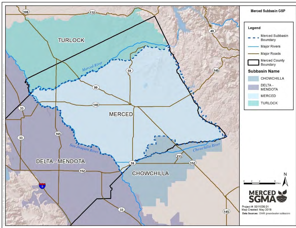
Figure 1-2: Neighboring Groundwater Subbasins
