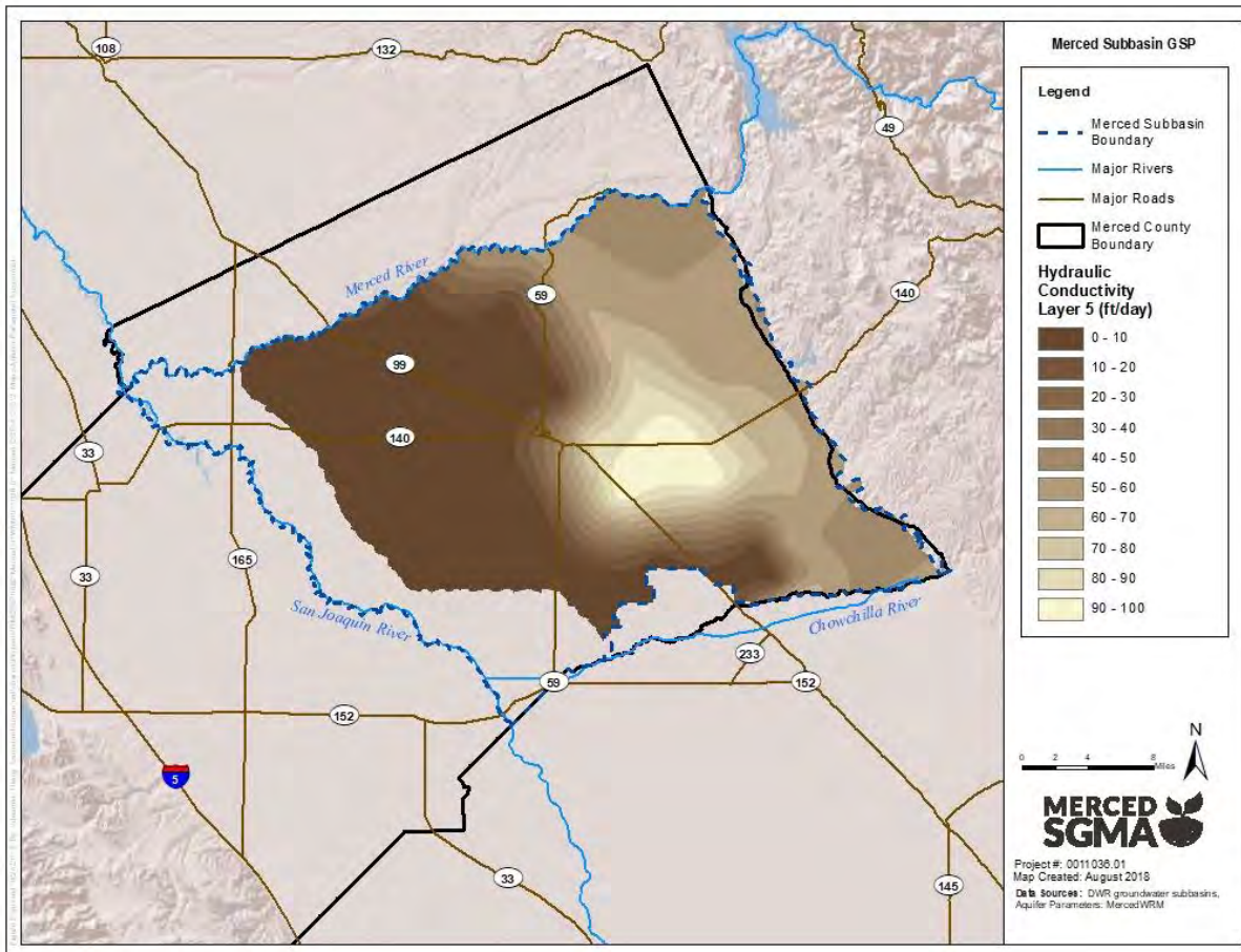
Figure 2-29: Hydraulic Conductivity – Mehrten Formation and Valley Springs Portion of Fractured Bedrock System (MercedWRM Layer 5)
