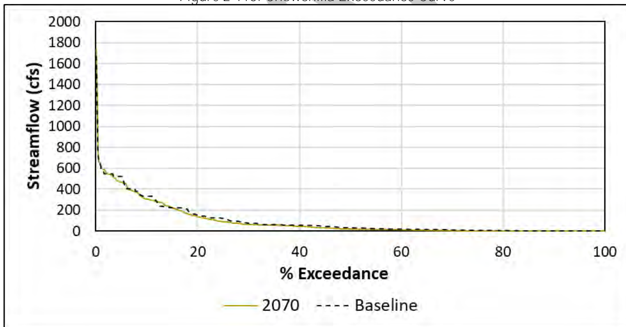
Figure 2-116: Chowchilla Exceedance Curve
