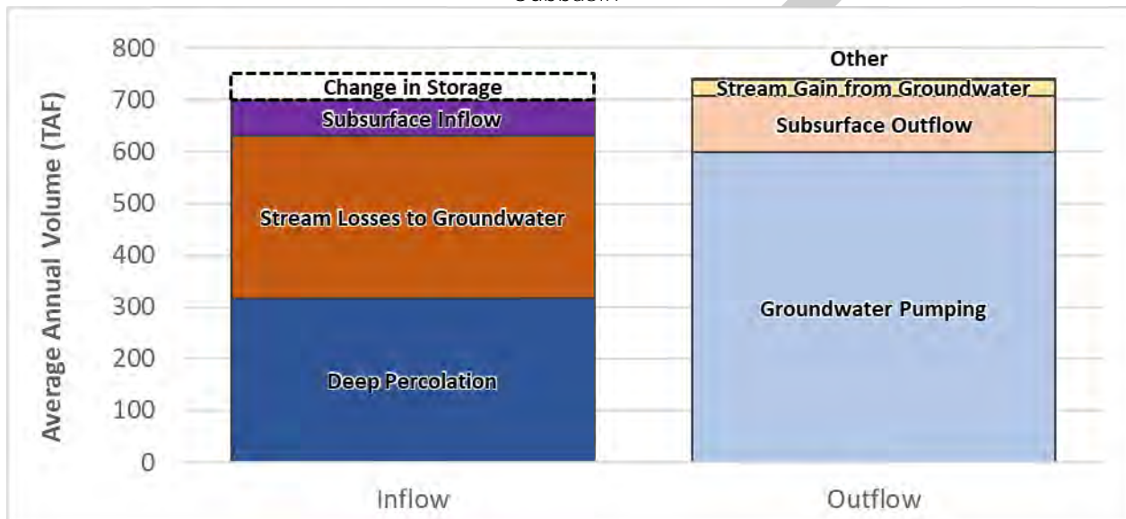
Figure 2-100: Current Conditions Annual Water Budget – Groundwater System, Merced Subbasin
