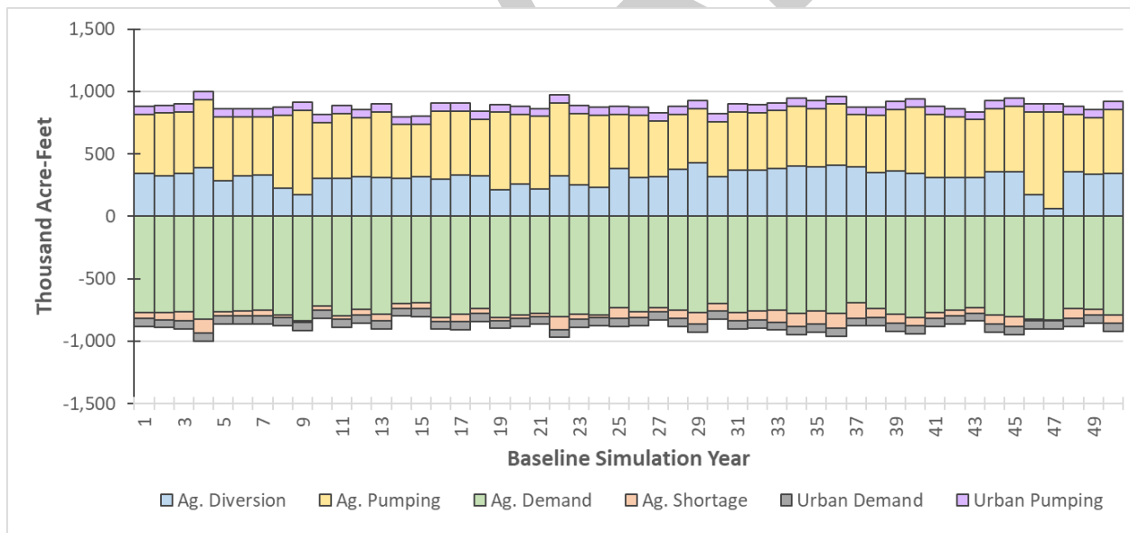
Figure 2-98: Current Conditions Annual Water Budget – Land Surface System, Merced Subbasin
