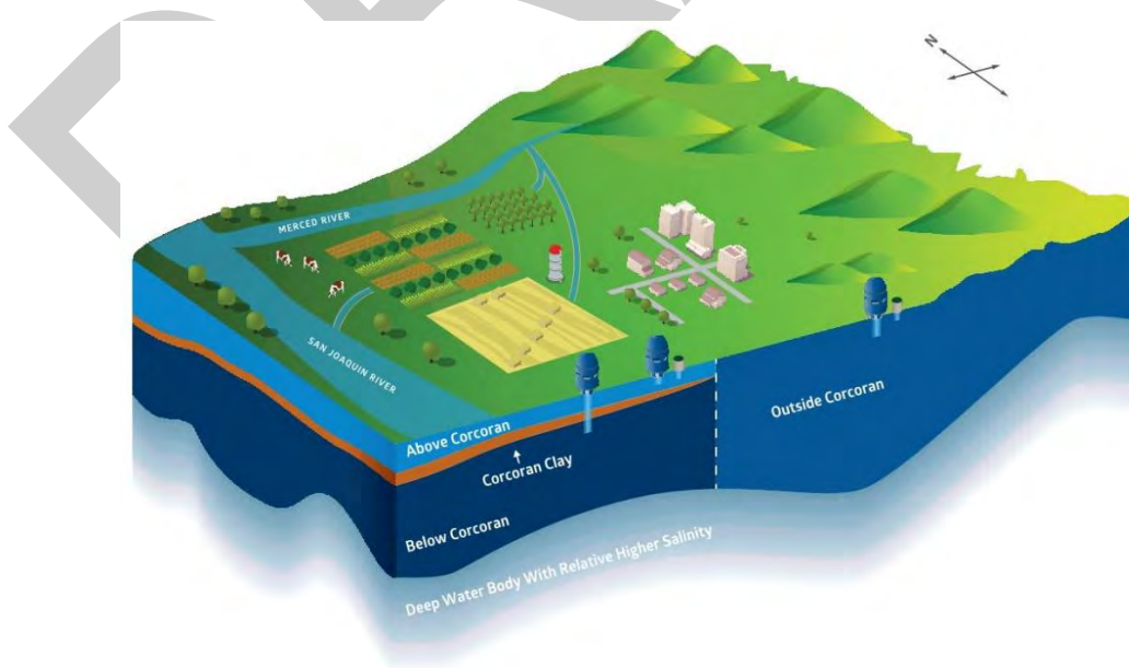
Figure ES-1-18: 3D Illustration of Merced Subbasin Principal Aquifers and Aquitard
