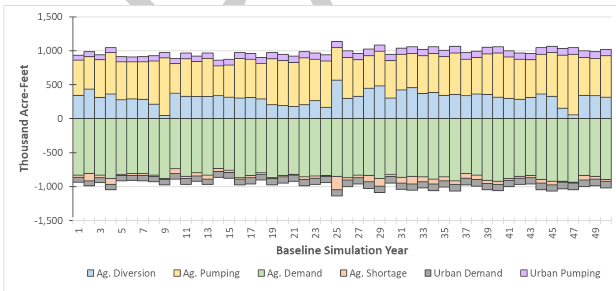
Figure 2-103: Projected Conditions Annual Water Budget – Land Surface System, Merced Subbasin
