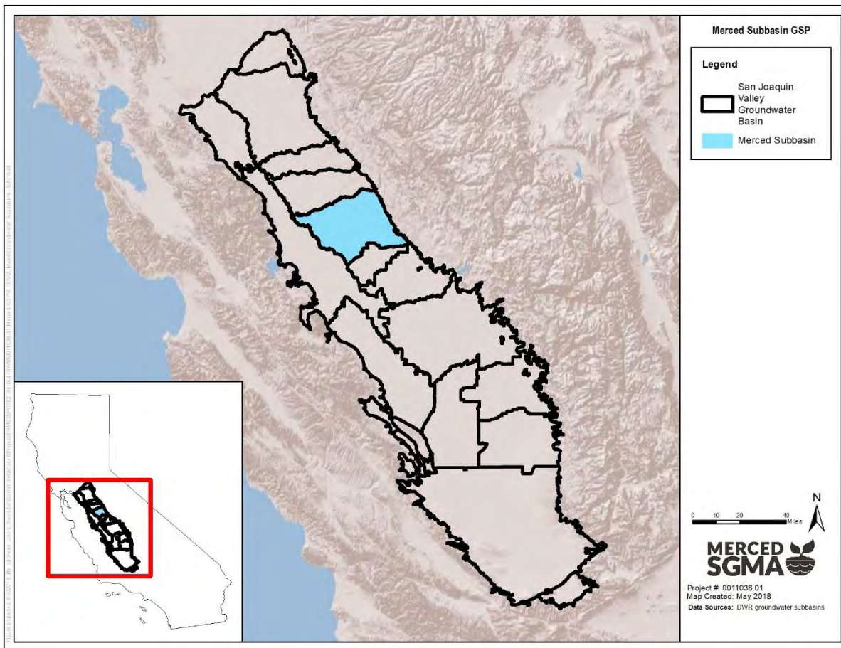
Figure 1-1: San Joaquin Valley Groundwater Basin
