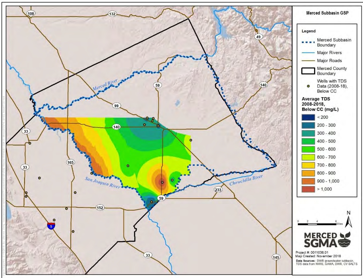
Figure 2-63: Average TDS Concentration 2008-2018, Below Corcoran Clay 1
