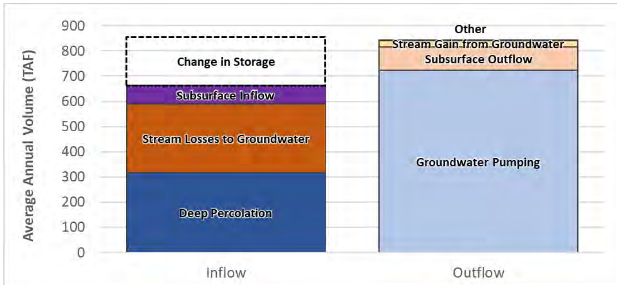
Figure 2-95: Historical Annual Water Budget – Groundwater System, Merced Subbasin
