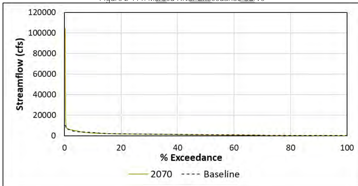
Figure 2-114: Merced River Exceedance Curve
