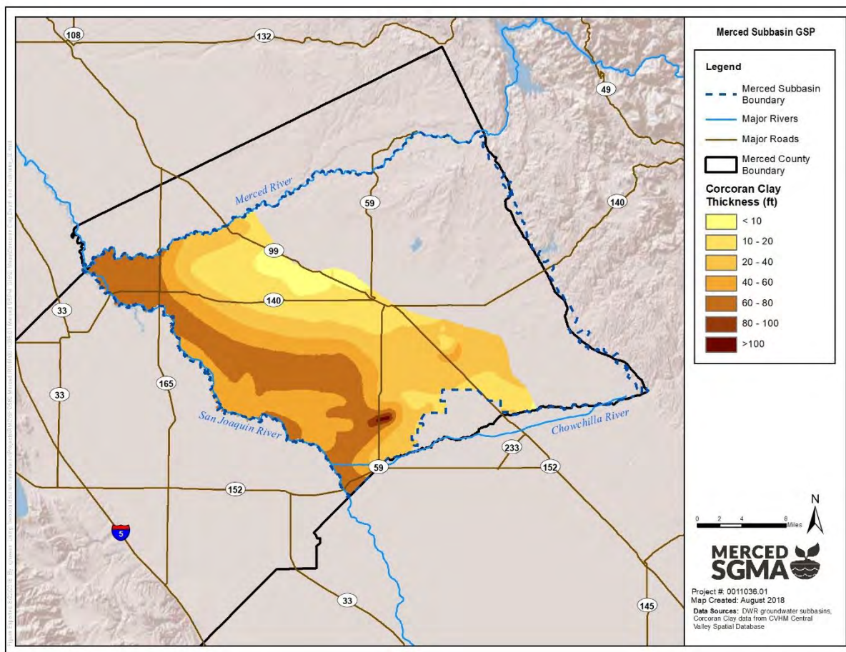
Figure 2-38: Corcoran Clay Thickness
