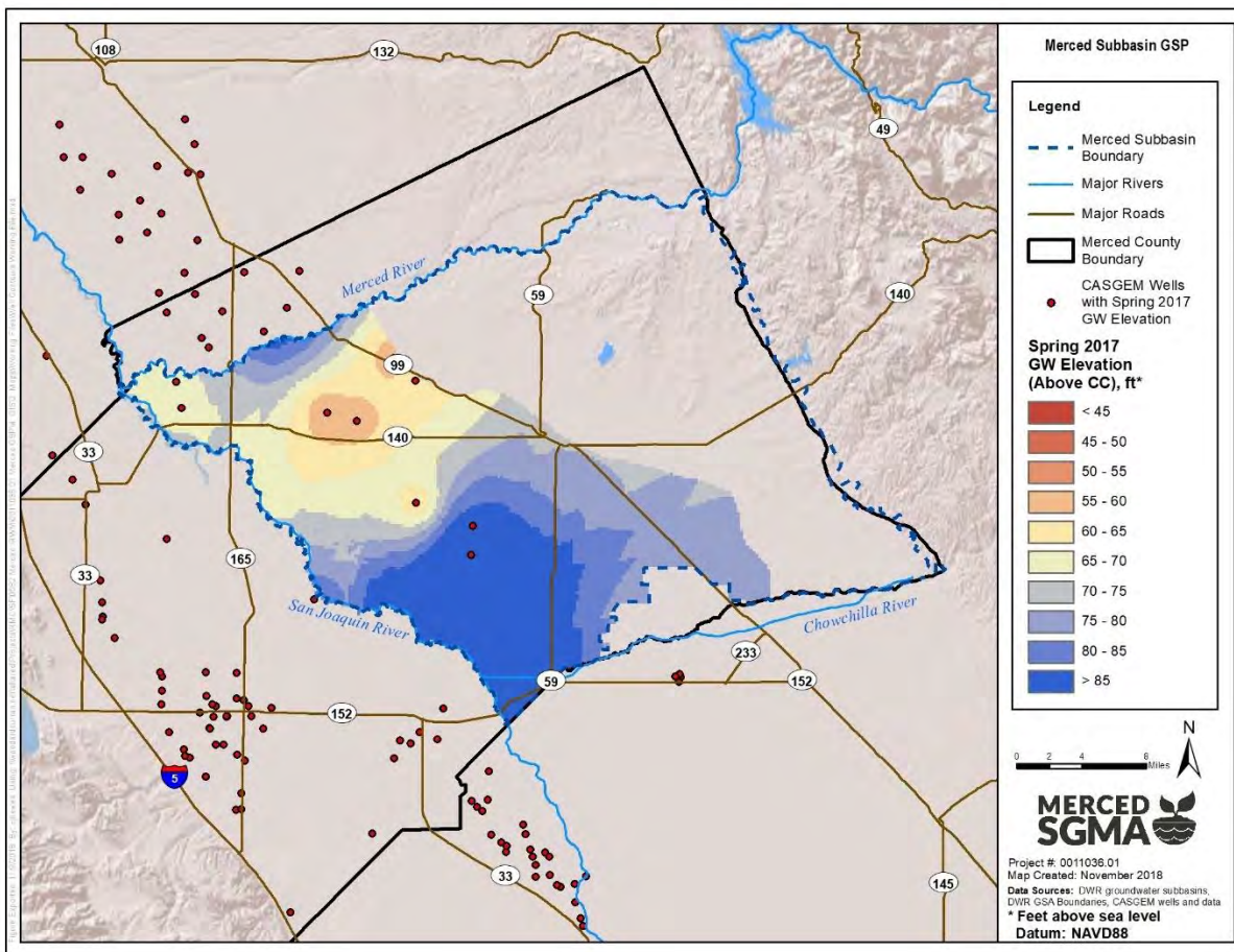
Figure 2-44: Spring 2017 Groundwater Elevation, Principal Aquifer: Above Corcoran Clay
