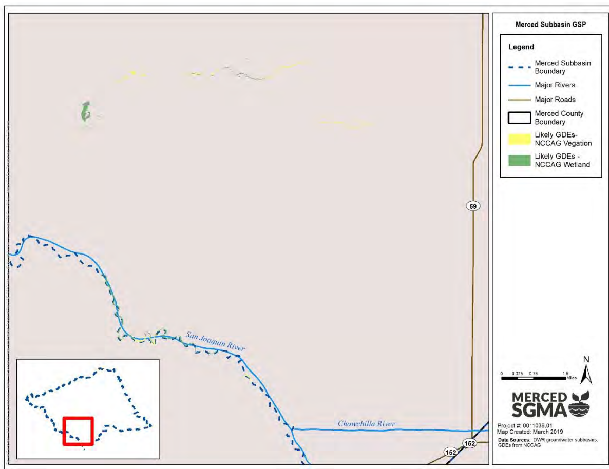
Figure 2-88: Likely GDEs – South Region of San Joaquin River
