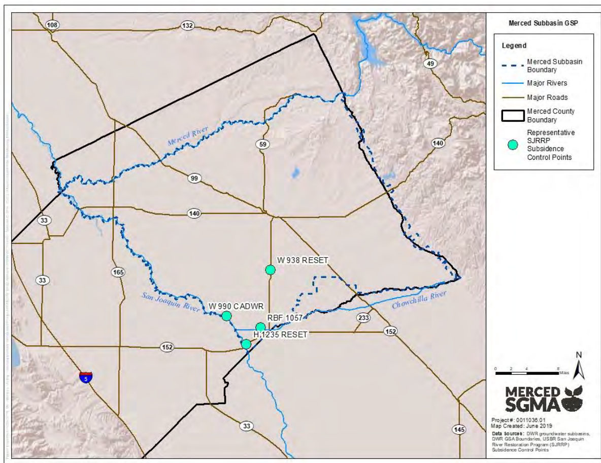
Figure 3-5: Minimum Threshold Subsidence Locations
