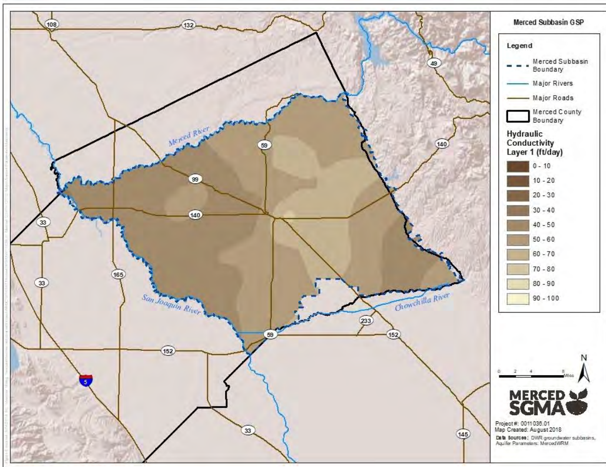
Figure 2-33: Hydraulic Conductivity – Shallow Unconfined Aquifer (MercedWRM Layer 1)
