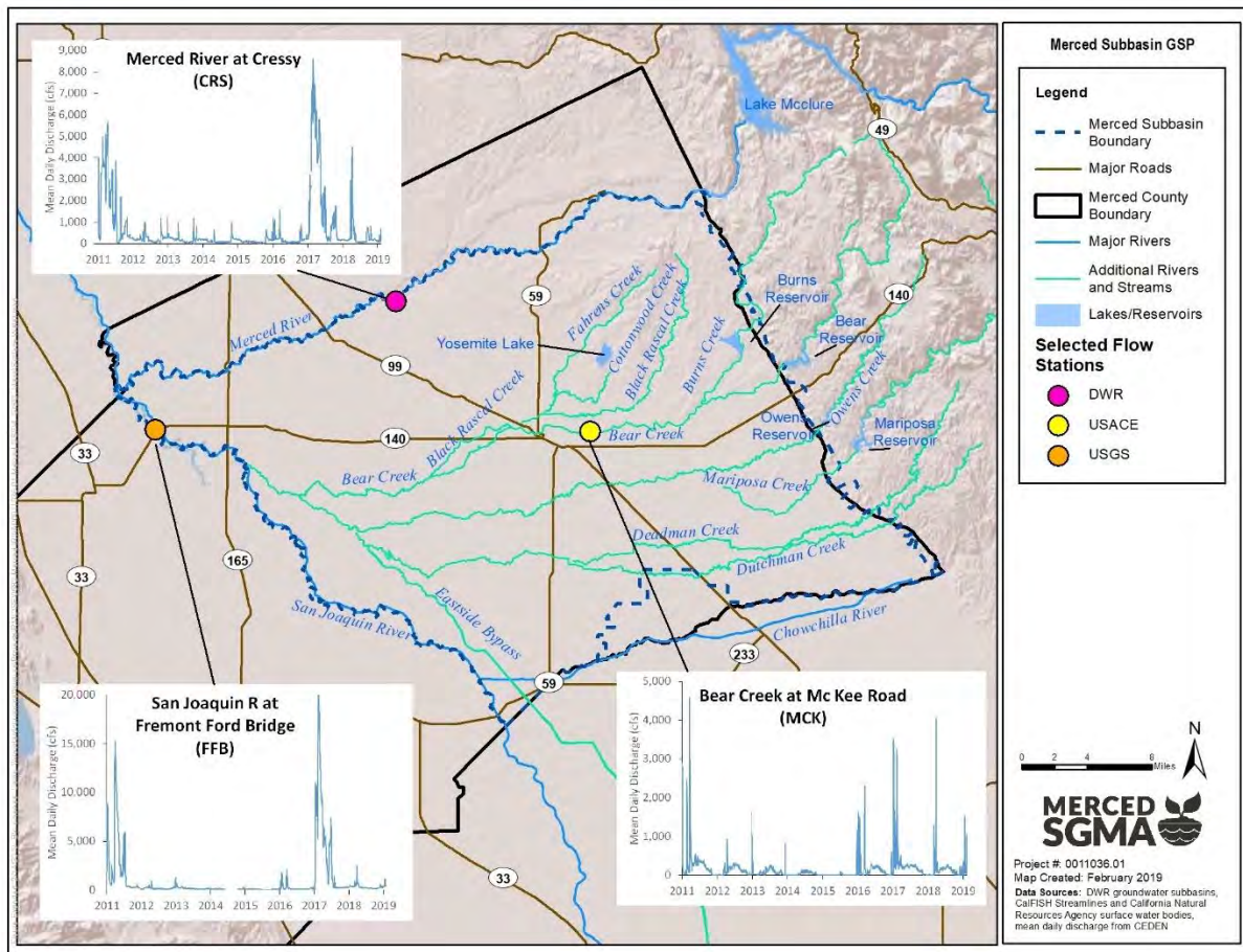
Figure 2-5: Surface Waters
