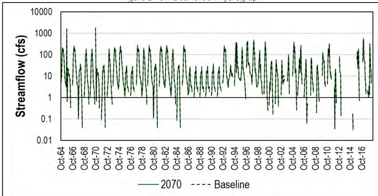
Figure 2-109: Bear Creek Hydrograph
