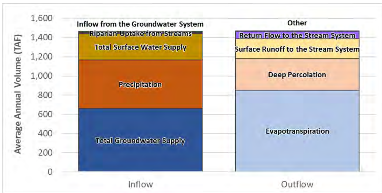
Figure 2-103: Projected Conditions Annual Water Budget – Land Surface System, Merced Subbasin
