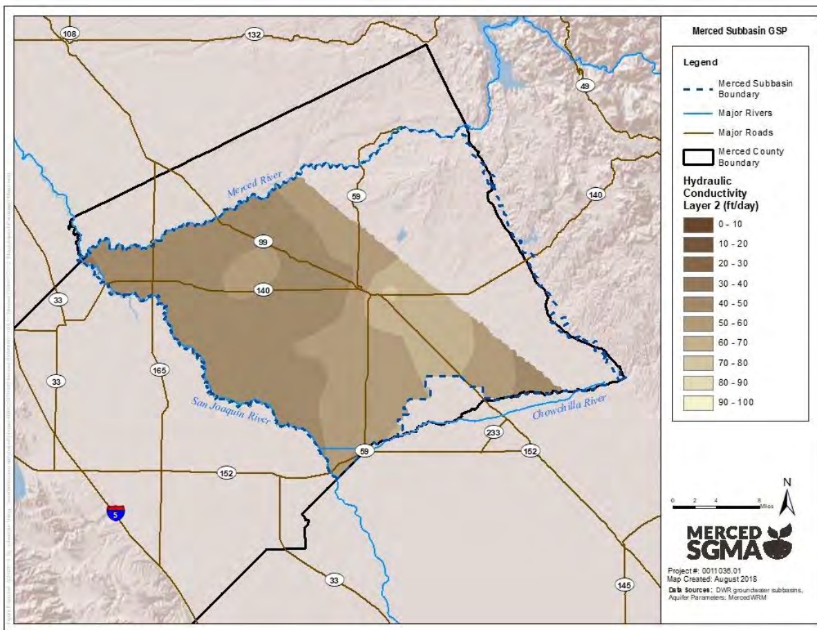
Figure 2-32: Hydraulic Conductivity – Intermediate Leaky-Aquifer (MercedWRM Layer 2)
