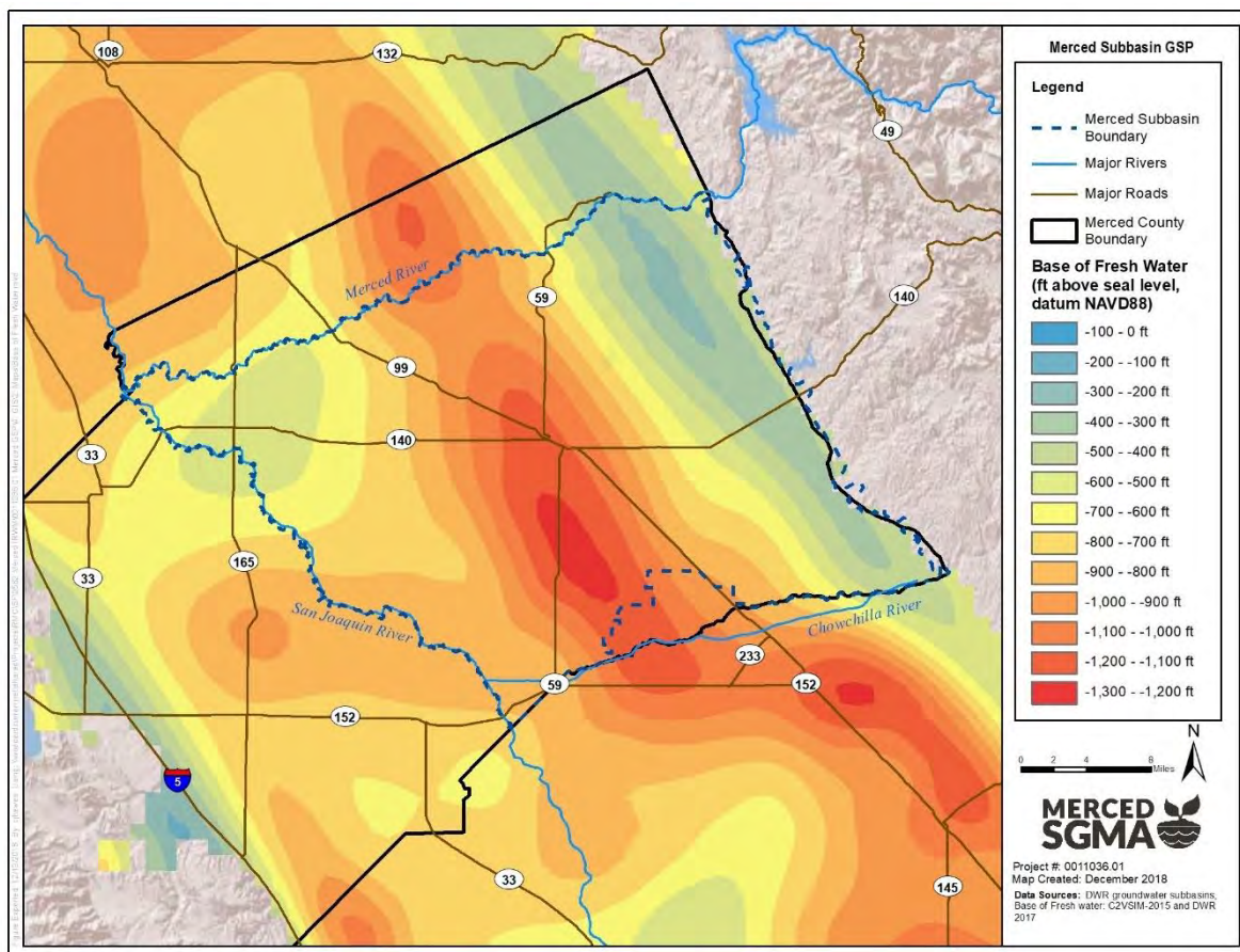
Figure 2-28: Base of Fresh Water
