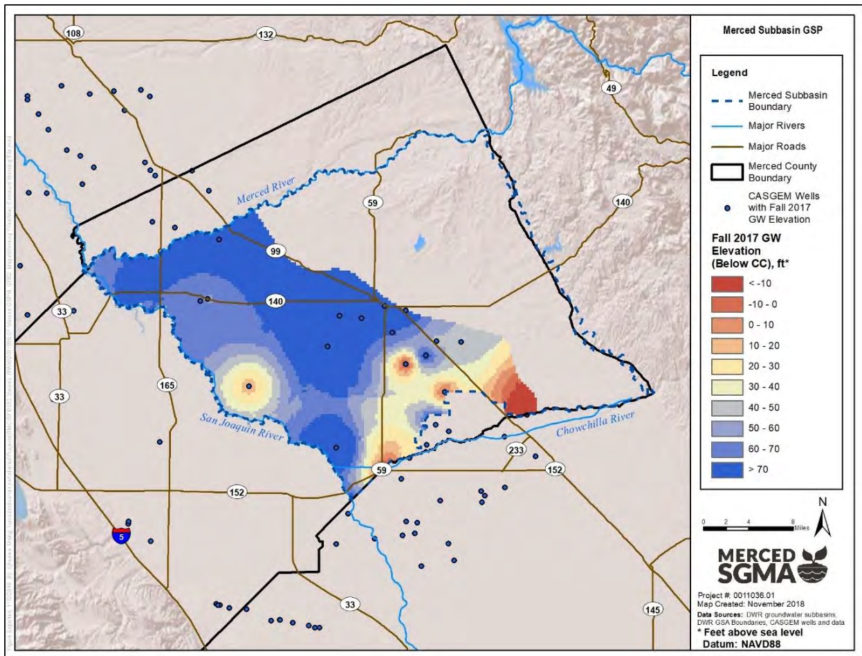
Figure 2-48: Fall 2017 Groundwater Elevation, Principal Aquifer: Below Corcoran Clay
