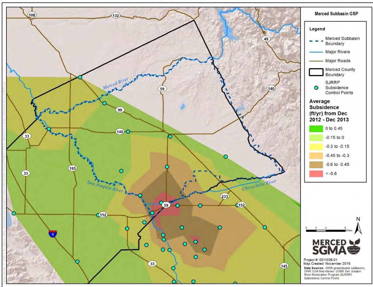
Figure 2-80: Land Subsidence December 2012 – December 2013
