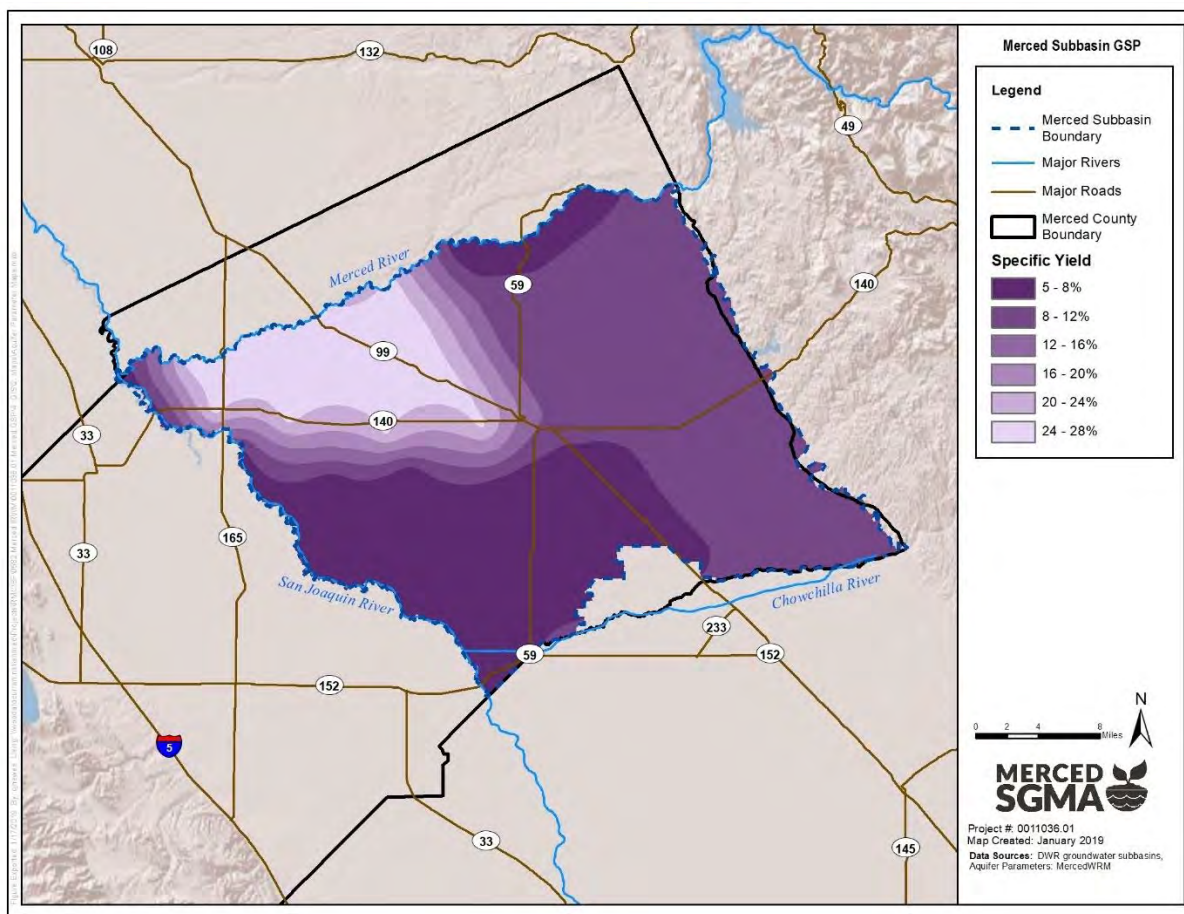
Figure 2-35: Specific Yield (all aquifer layers)
