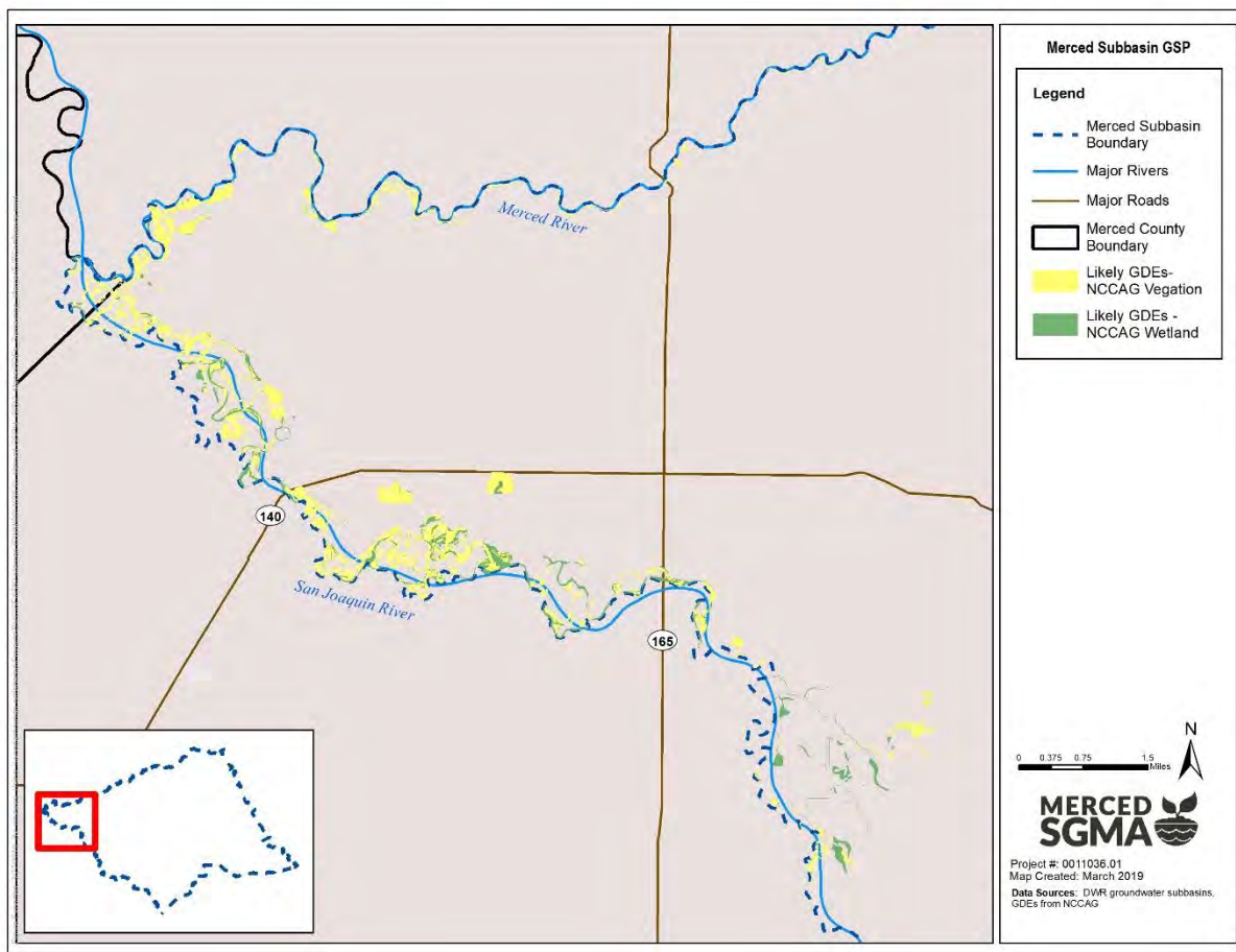
Figure 2-87: Likely GDEs – Confluence of Merced and San Joaquin Rivers
