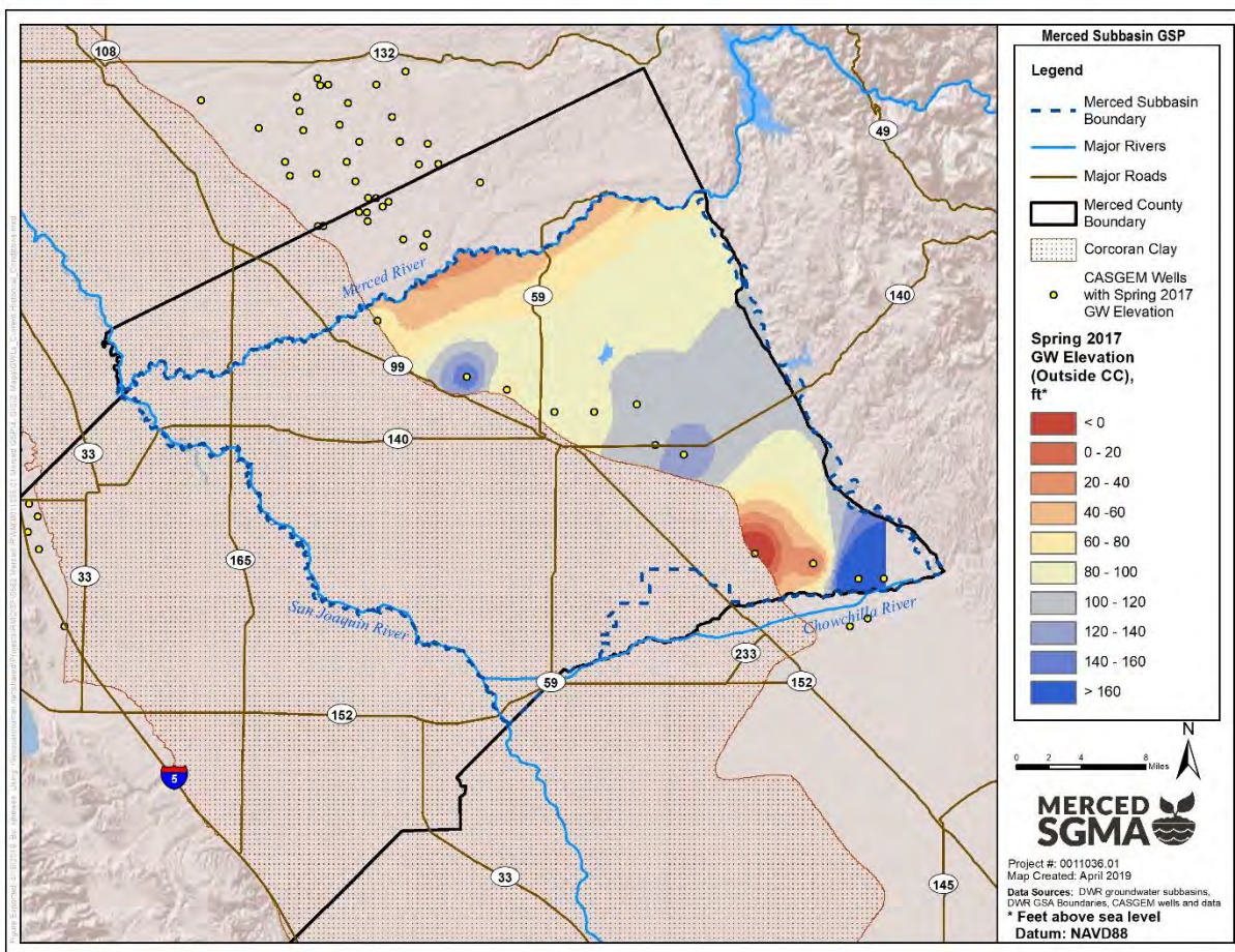
Figure 2-46: Spring 2017 Groundwater Elevation, Principal Aquifer: Outside Corcoran Clay
