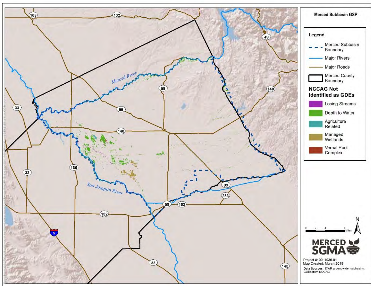
Figure 2-86: NCCAG Not Identified as GDEs ▲
