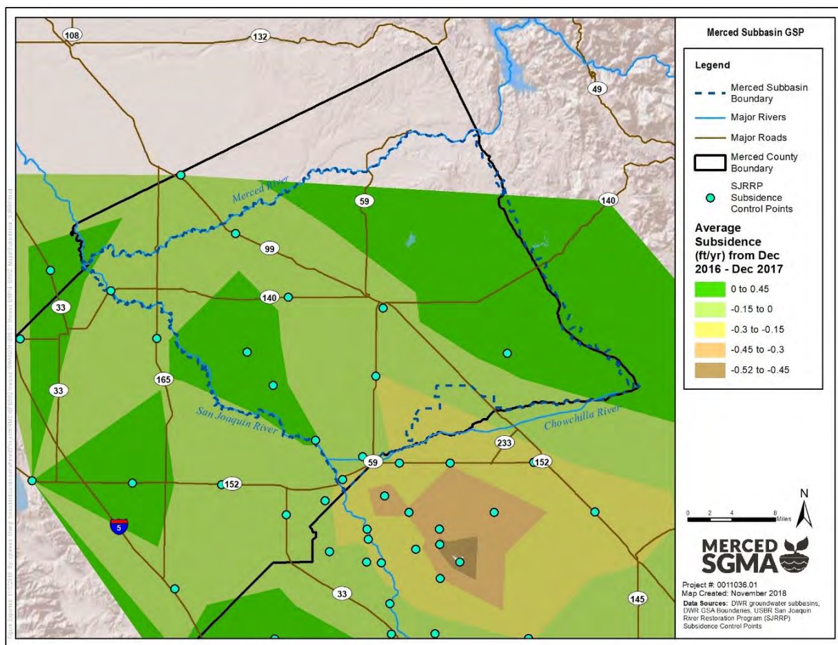
Figure 2-81: Land Subsidence December 2016 – December 2017
