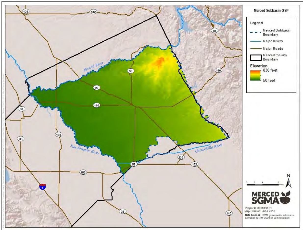
Figure 2-1: Topography
