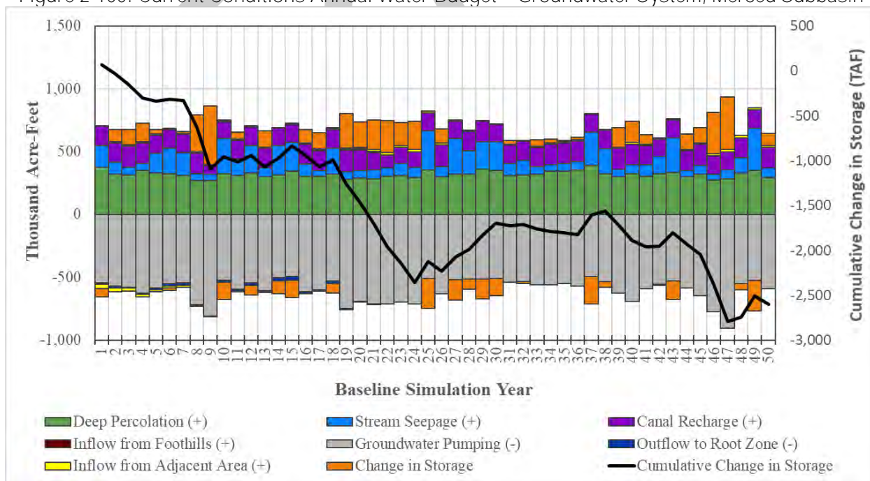
Figure 2-100: Current Conditions Annual Water Budget – Groundwater System, Merced Subbasin
