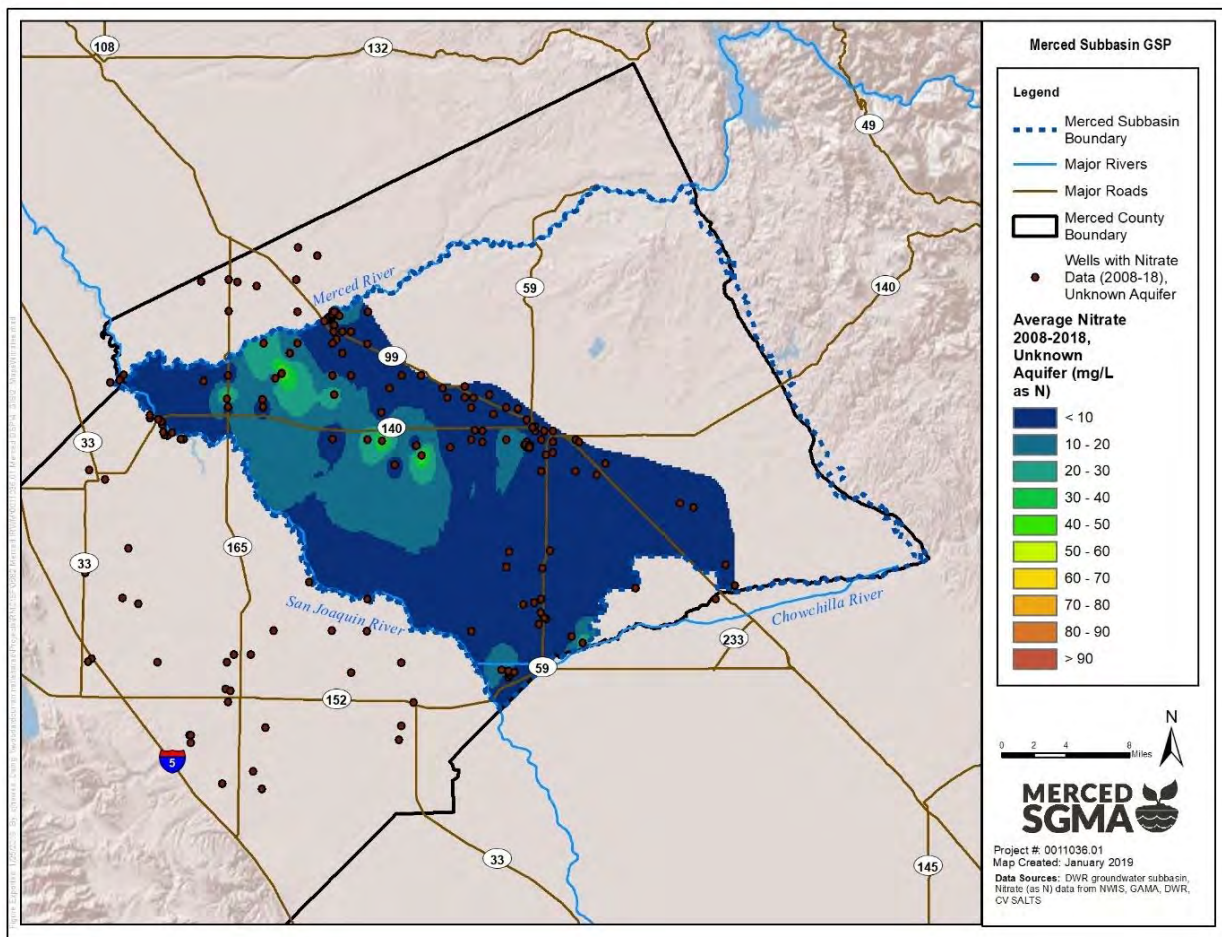
Figure 2-61: Average Nitrate Concentration 2008-2018, Unknown Aquifer
