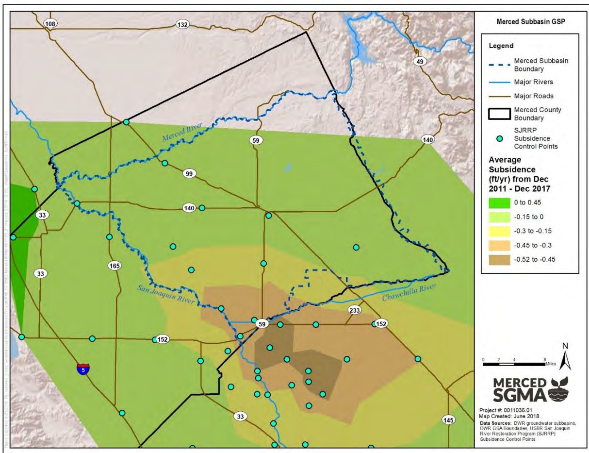
Figure 2-79: Average Land Subsidence December 2011 – December 2017
