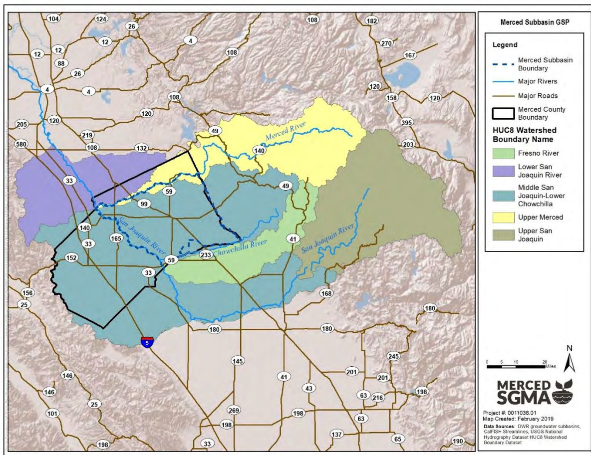
Figure 2-7: HUC8 Watershed Boundaries
