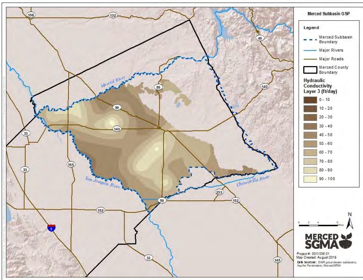
Figure 2-31: Hydraulic Conductivity – Confined Aquifer (MercedWRM Layer 3)
