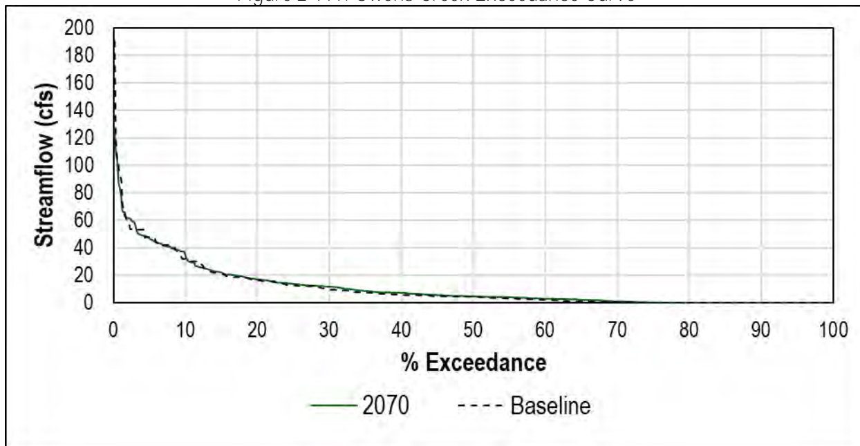
Figure 2-111: Owens Creek Exceedance Curve
