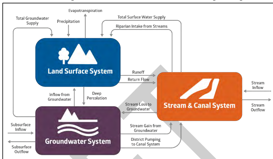
Figure ES-1-19: Generalized Water Budget Diagram
