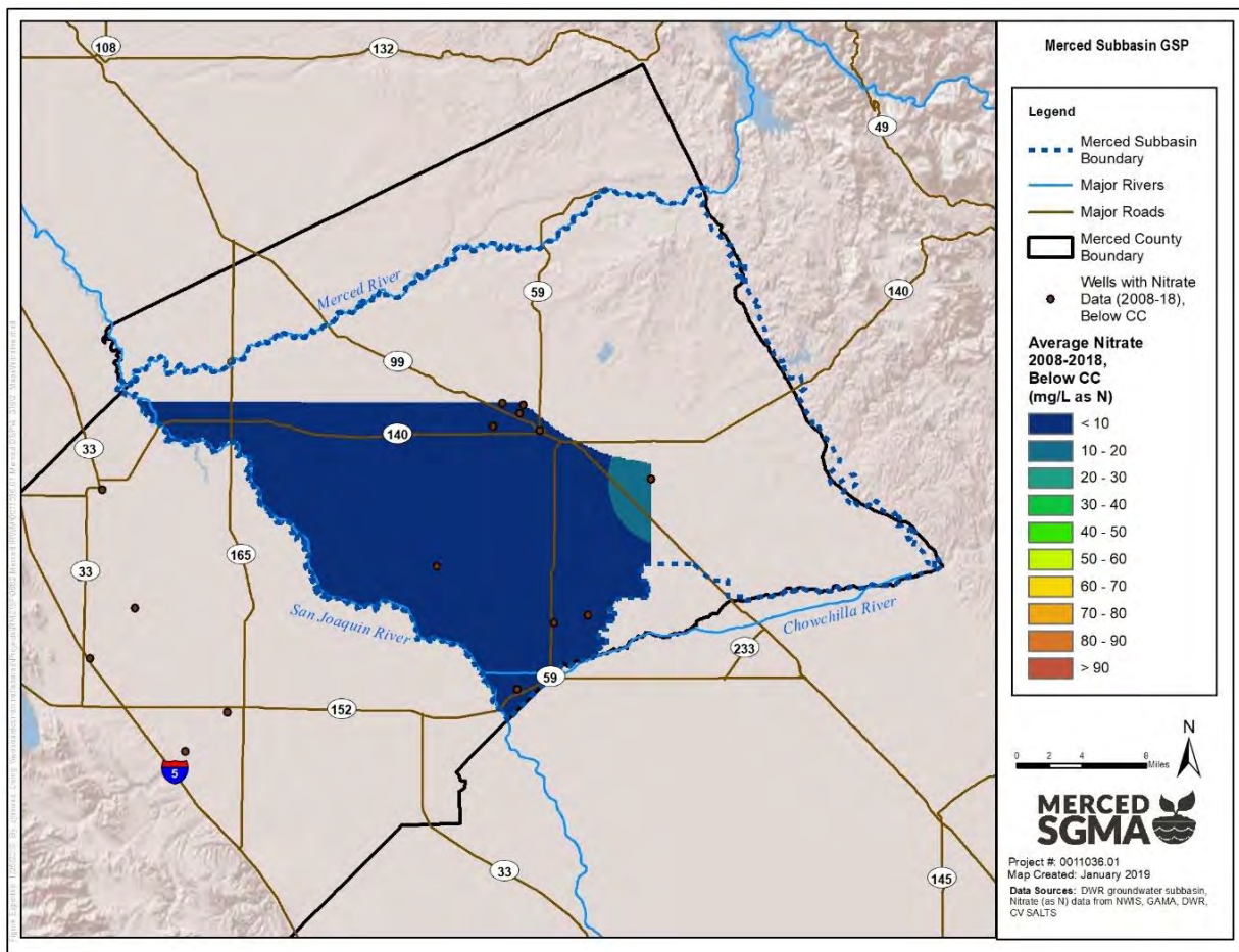
Figure 2-60: Average Nitrate Concentration 2008-2018, Below Corcoran Clay 1
