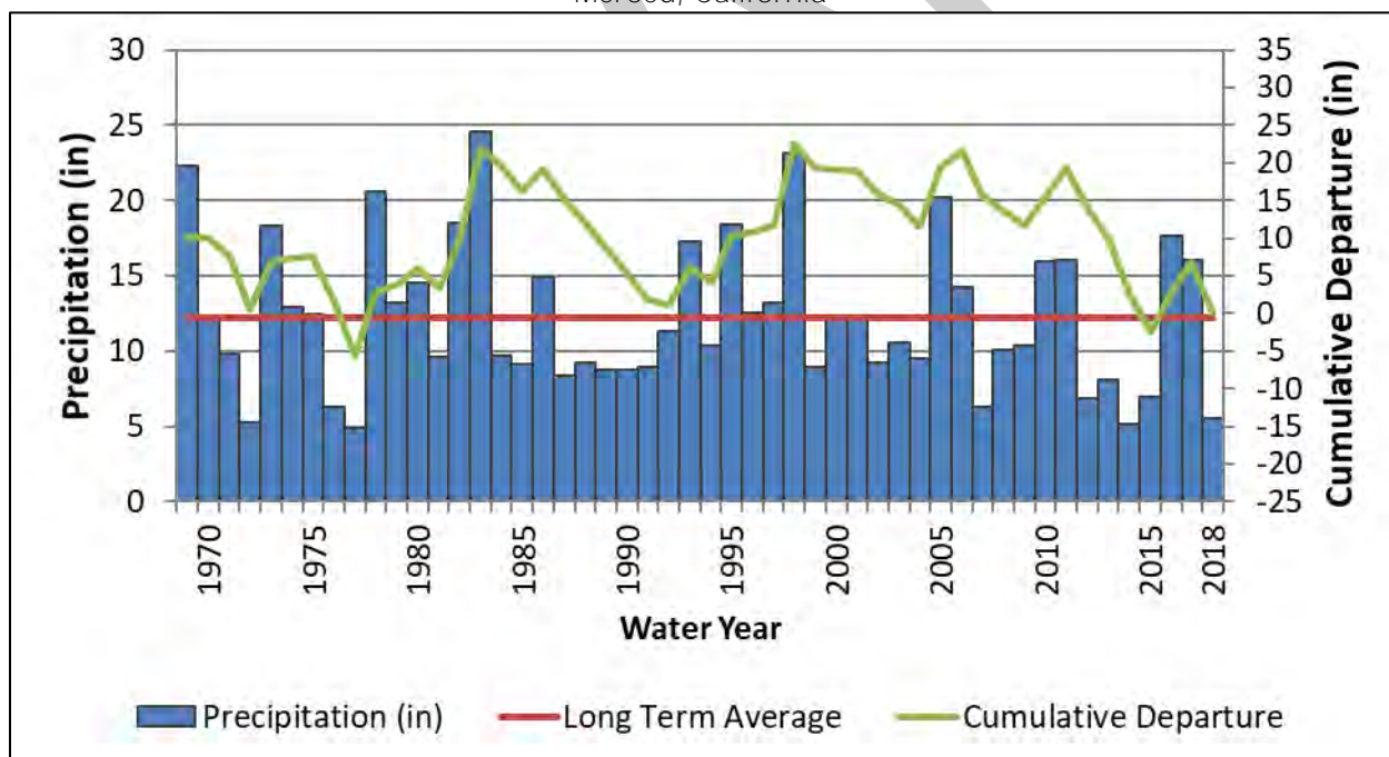
Figure 2-90: 50-Year Historical Precipitation and Cumulative Departure from Mean Precipitation, Merced, California
