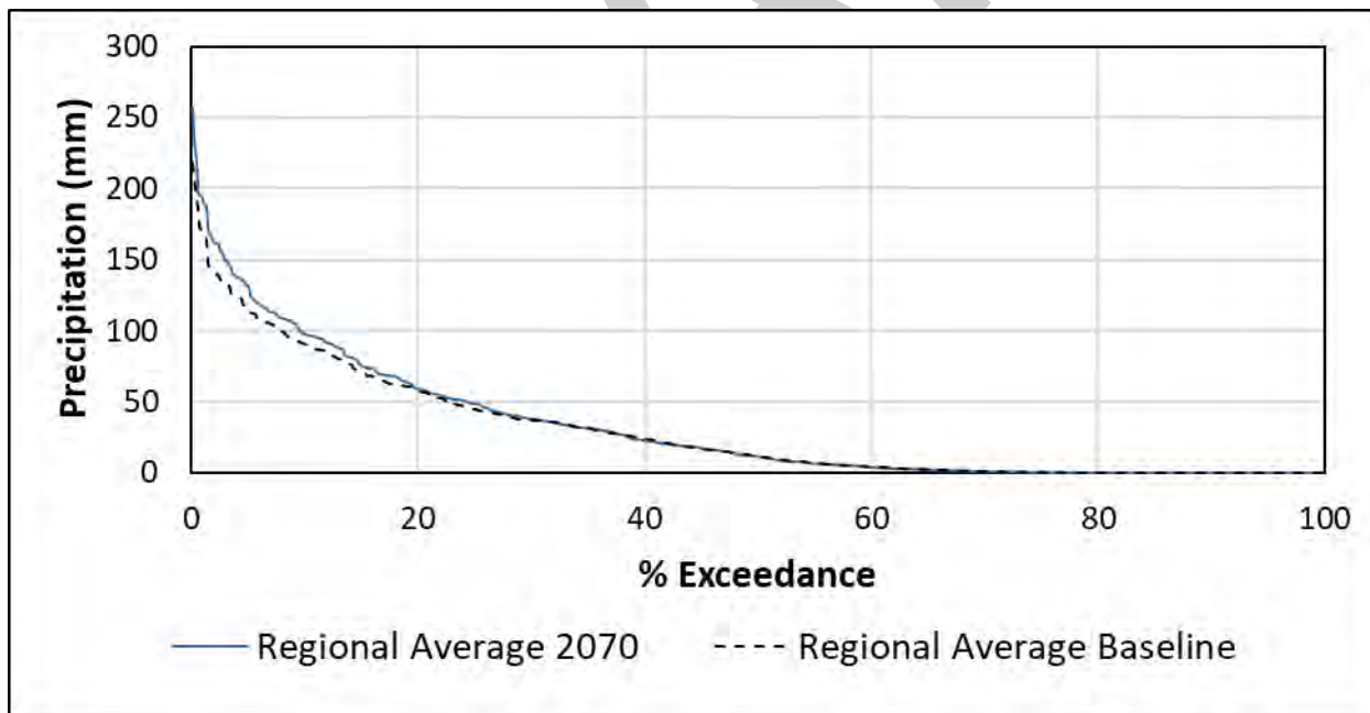
Figure 2-120: Perturbed Precipitation Exceedance Curve
