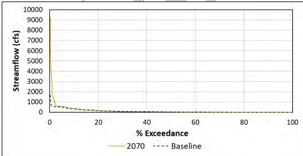
Figure 2-118: San Joaquin River Exceedance Curve
