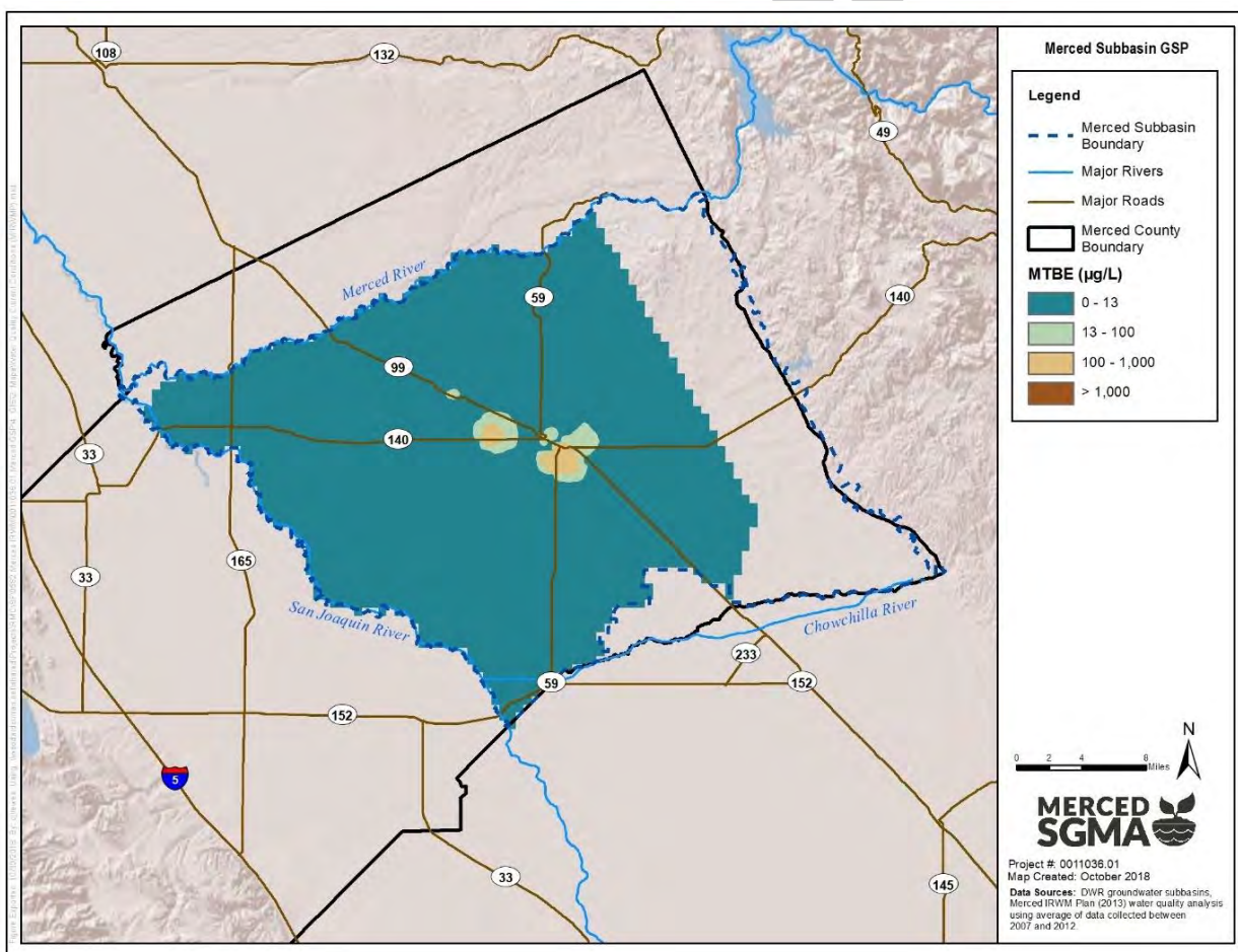
Figure 2-75: 5-Year Average Distribution of MTBE in Groundwater (2012-2017)
