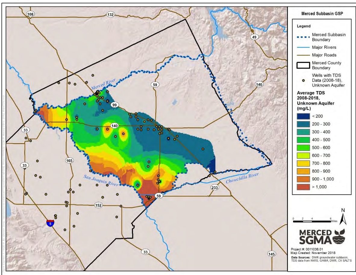
Figure 2-64: Average TDS Concentration 2008-2018, Unknown Aquifer
