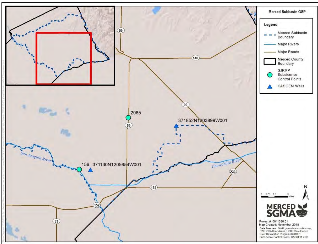
Figure 2-82: Map of Subsidence and Groundwater Well Comparison Points
