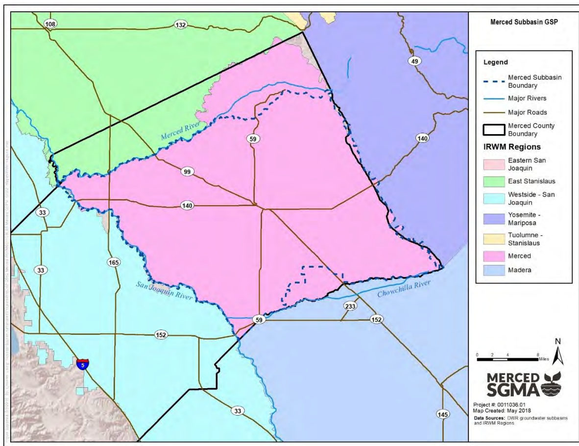
Figure 1-10: Merced IRWM Region Setting
