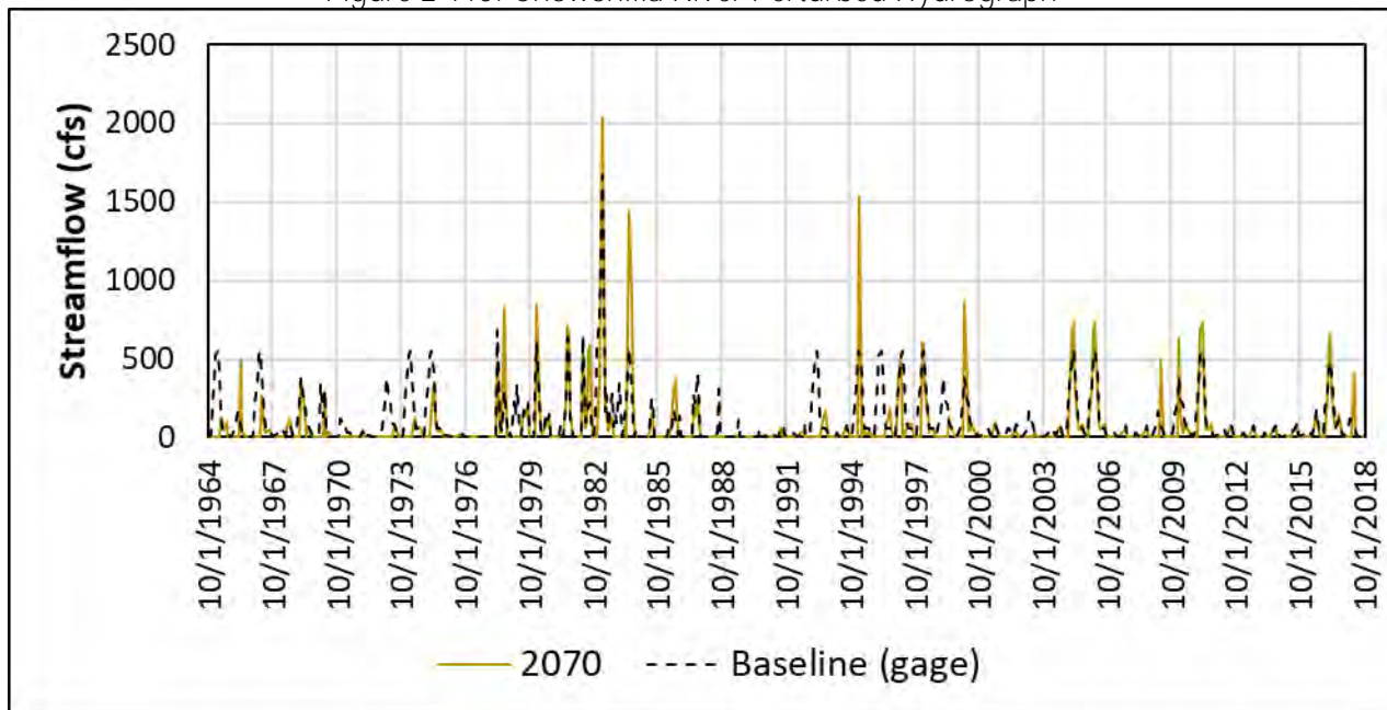
Figure 2-115: Chowchilla River Perturbed Hydrograph
