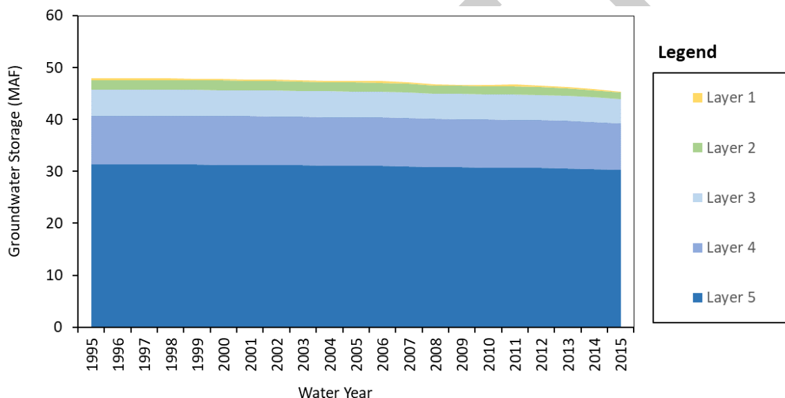
Figure 2-57: Historical Modeled Change in Storage by MercedWRM Layer
