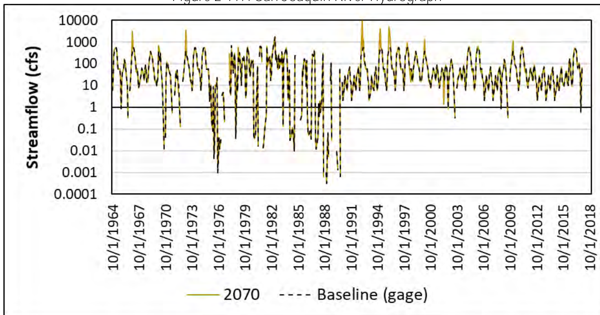
Figure 2-117: San Joaquin River Hydrograph
