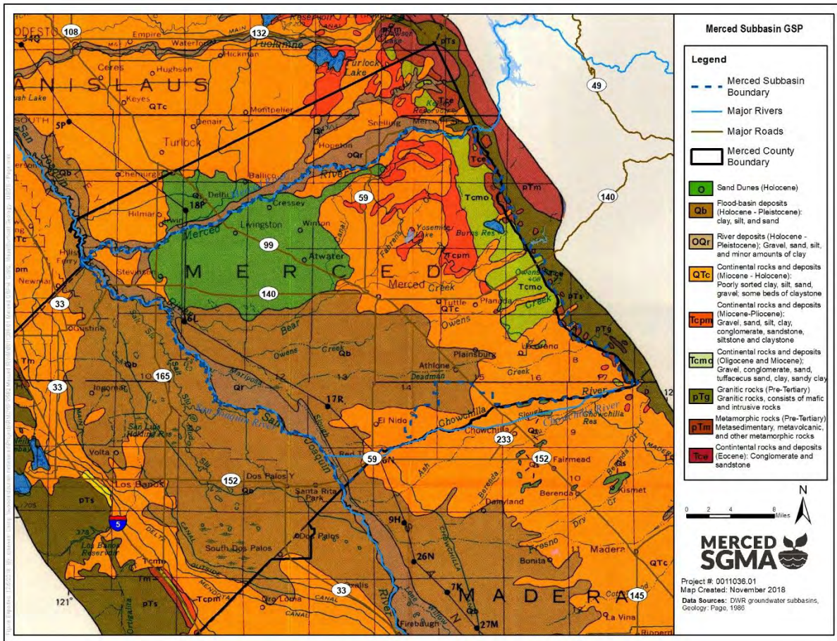
Figure 2-11: Surficial Geology
