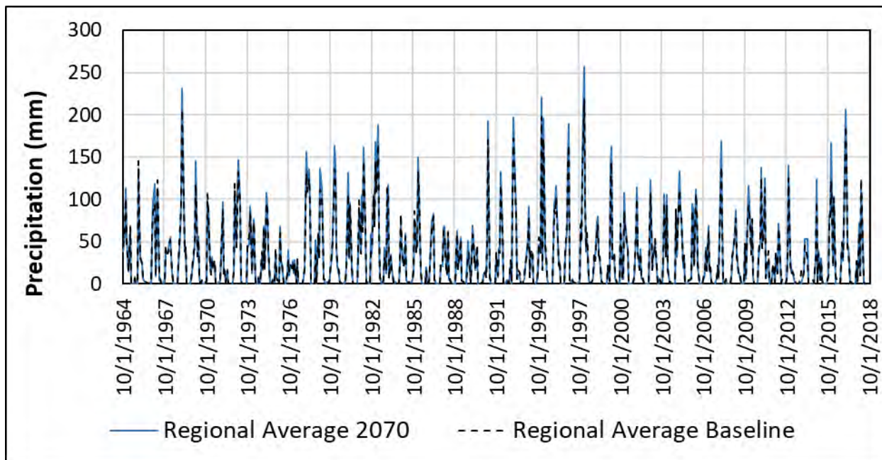
Figure 2-119: Perturbed Precipitation Under Climate Change
