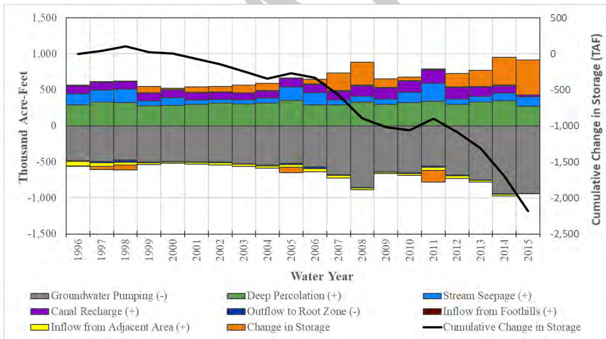
Figure 2-95: Historical Annual Water Budget – Groundwater System, Merced Subbasin
