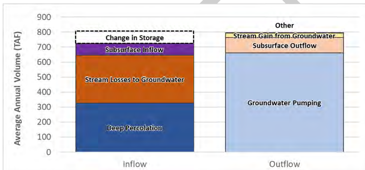
Figure 2-104: Projected Conditions Average Annual Water Budget – Groundwater System, Merced Subbasin
