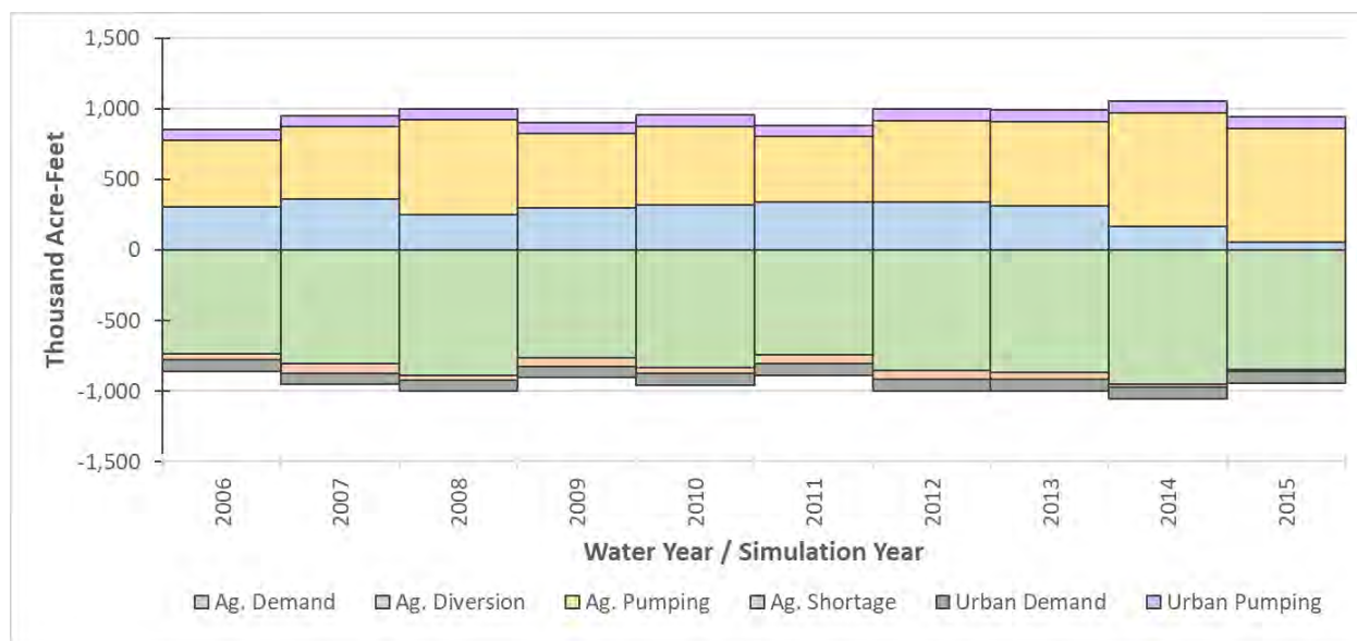
Figure 2-93: Historical Annual Water Budget – Land Surface System, Merced Subbasin
