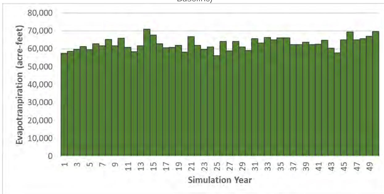
Figure 2-123: Simulated changes in Evapotranspiration due to Climate Change (Scenario minus Baseline)
