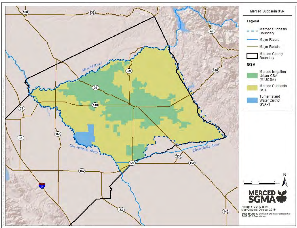
Figure 1-5: GSA Boundaries
