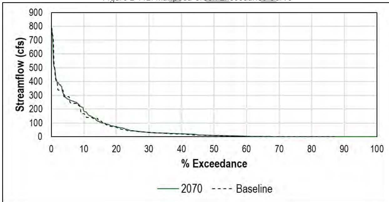
Figure 2-112: Mariposa Creek Exceedance Curve
