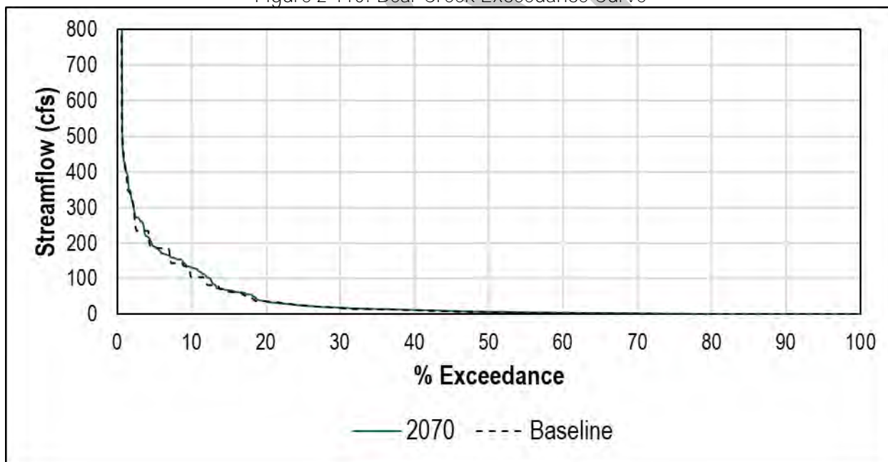
Figure 2-110: Bear Creek Exceedance Curve
