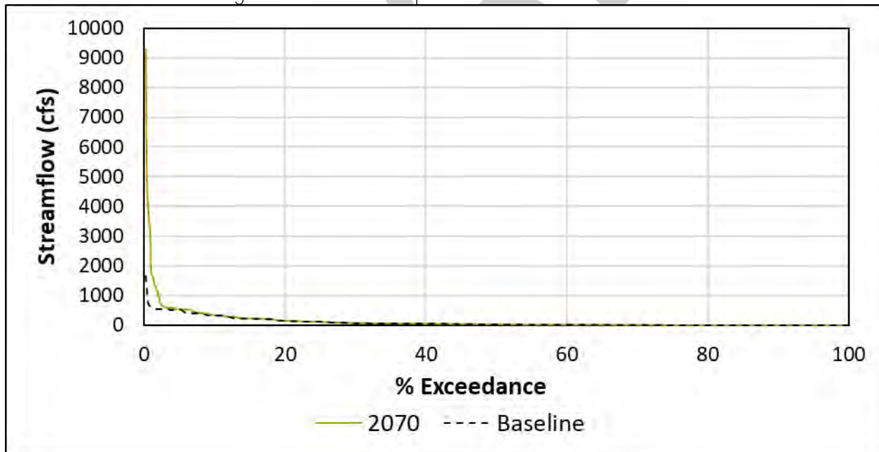
Figure 2-111: San Joaquin River Exceedance Curve
