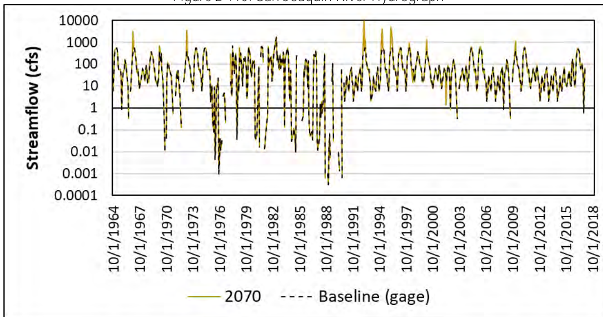
Figure 2-110: San Joaquin River Hydrograph
