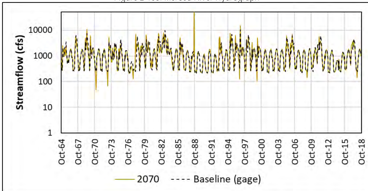
Figure 2-106: Merced River Hydrograph
