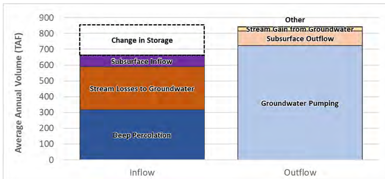
Figure 2-93: Historical Average Annual Water Budget – Groundwater System, Merced Subbasin
