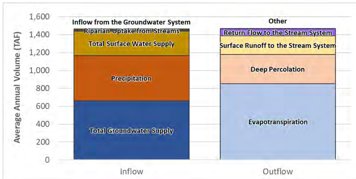
Figure 2-98: Projected Conditions Average Annual Water Budget – Land Surface System, Merced Subbasin
