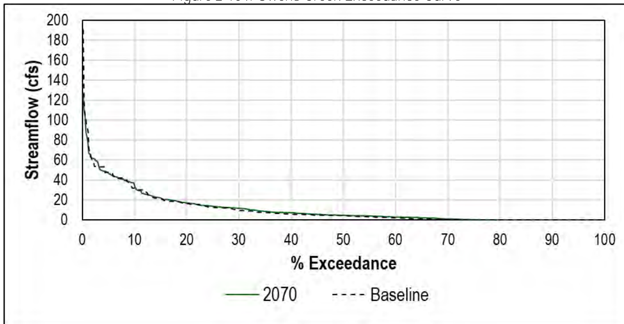
Figure 2-104: Owens Creek Exceedance Curve
