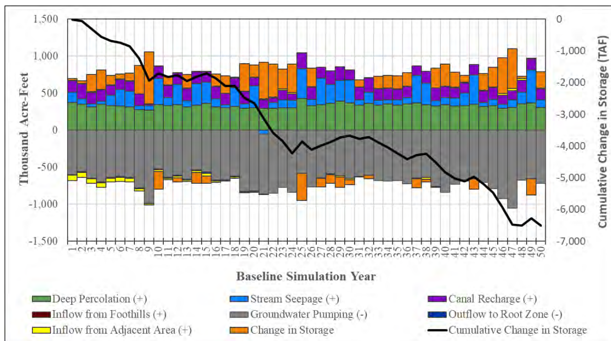
Figure 2-120: Groundwater Budget - MercedWRM Climate Change Scenario
