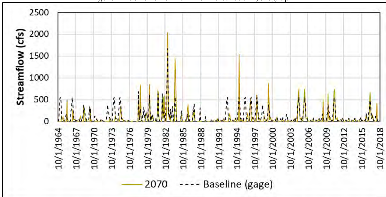
Figure 2-108: Chowchilla River Perturbed Hydrograph
