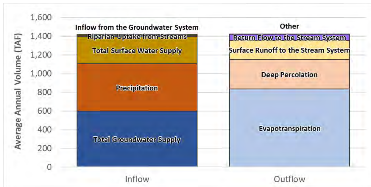
Figure 2-95: Current Conditions Average Annual Water Budget – Land Surface System, Merced Subbasin
