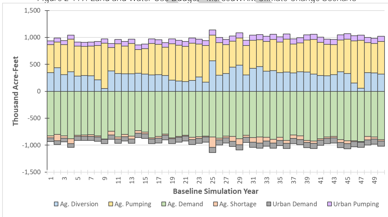
Figure 2-119: Land and Water Use Budget - MercedWRM Climate Change Scenario
