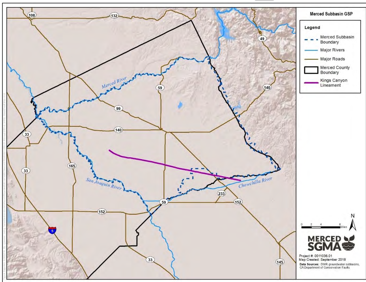
Figure 2-26: Fault Map
