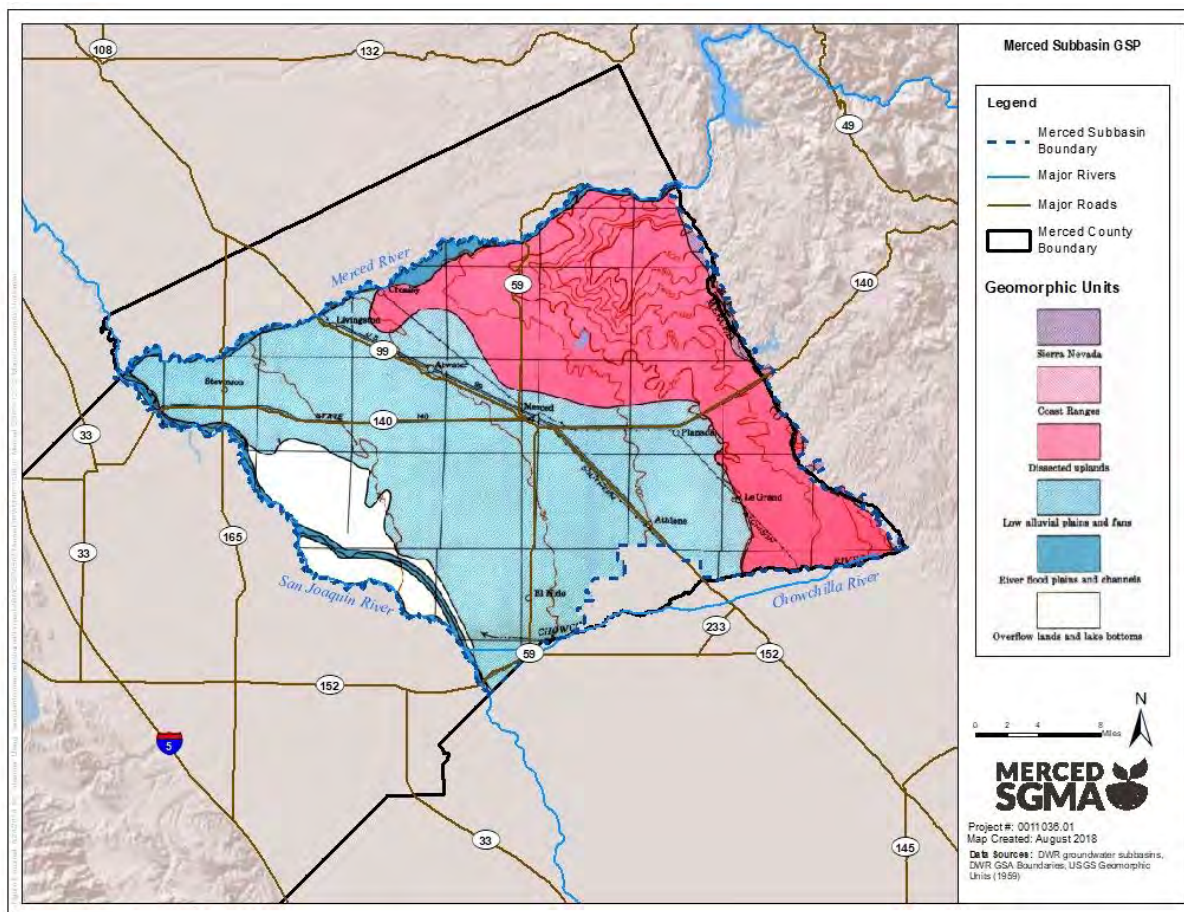
Figure 2-2: Geomorphic Units
