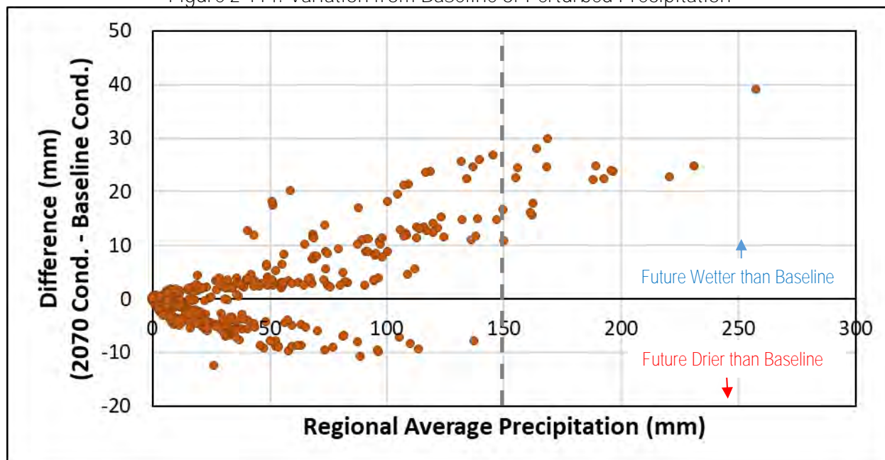
Figure 2-114: Variation from Baseline of Perturbed Precipitation
