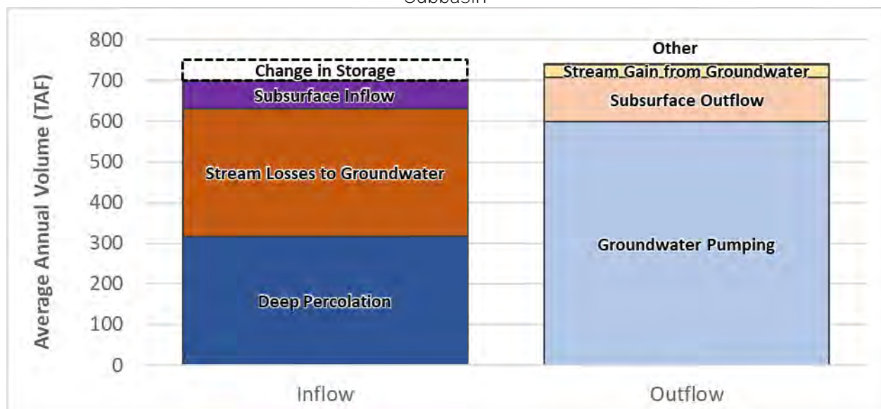
Figure 2-96: Current Conditions Average Annual Water Budget – Groundwater System, Merced Subbasin
