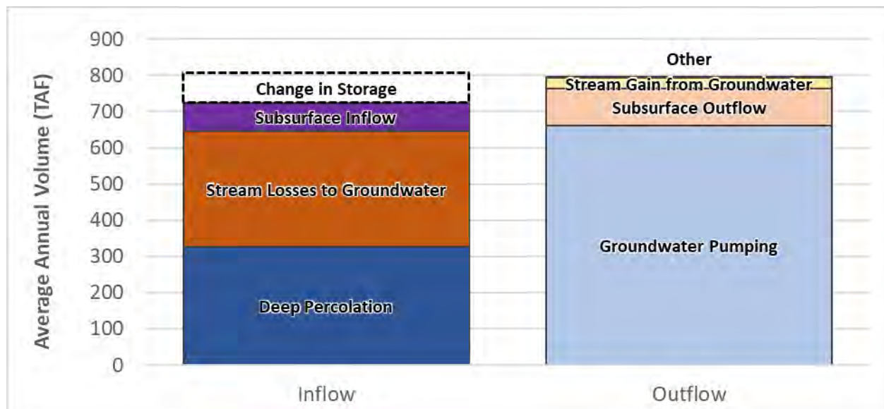
Figure 2-99: Projected Conditions Average Annual Water Budget – Groundwater System, Merced Subbasin
