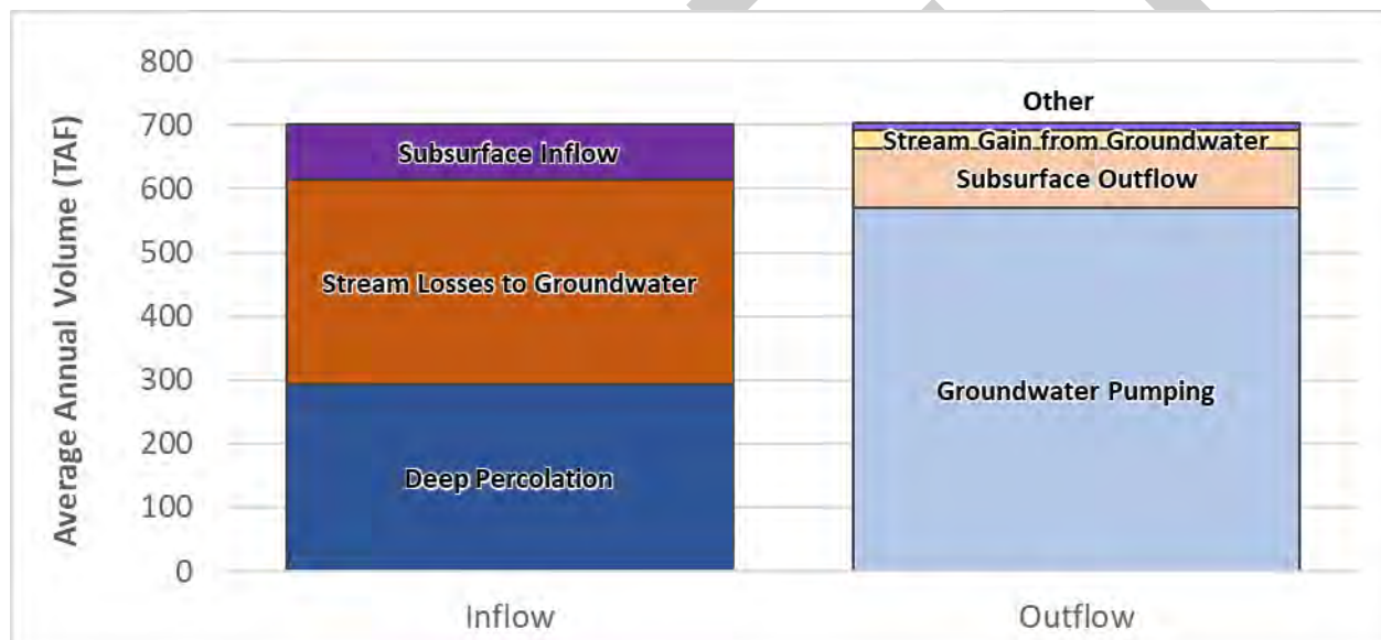
Figure 2-100: Groundwater Water Budget under Sustainable Groundwater Management Conditions Long-Term (50-Year) Average Annual
