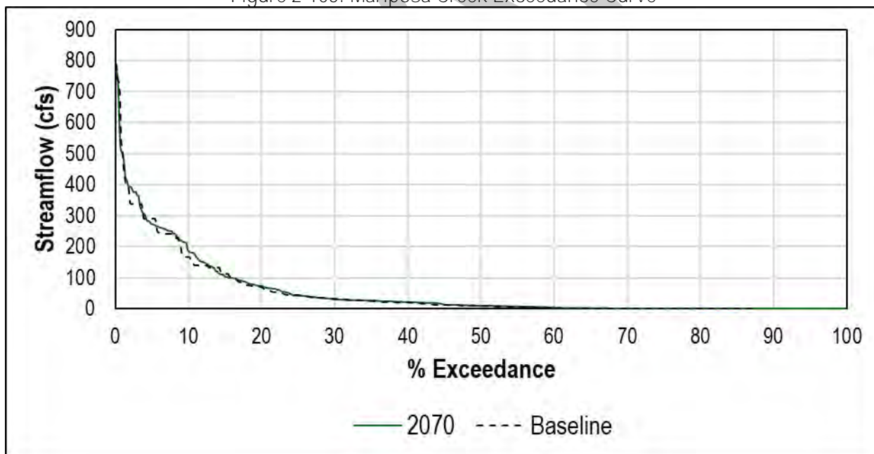
Figure 2-105: Mariposa Creek Exceedance Curve
