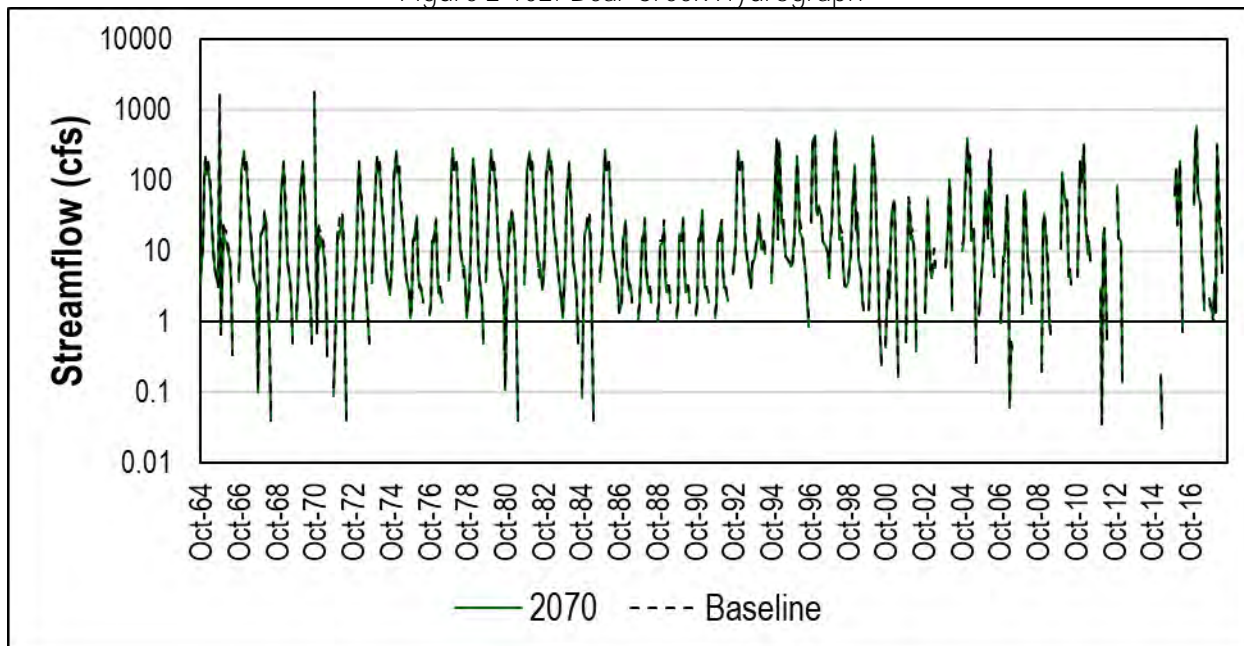
Figure 2-102: Bear Creek Hydrograph
