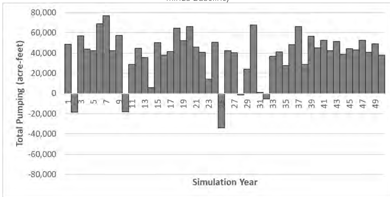
Figure 2-118: Simulated Changes in Groundwater Production due to Climate Change (Scenario minus Baseline)
