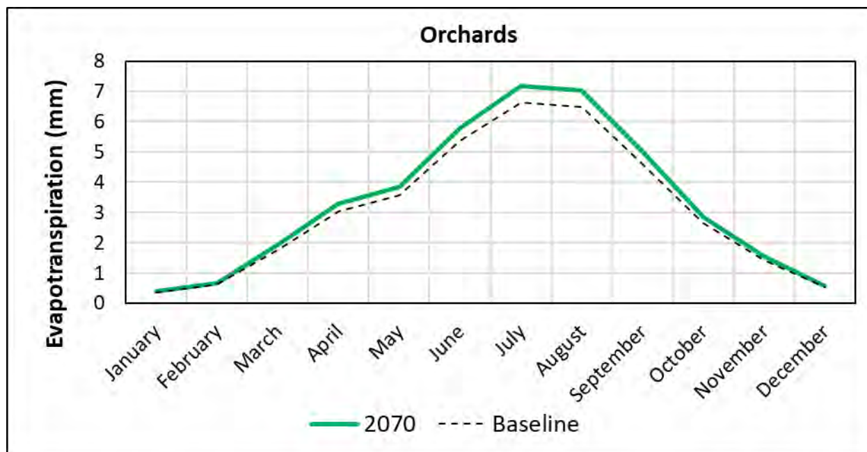
Figure 2-115: Monthly ET for Sample Crops
