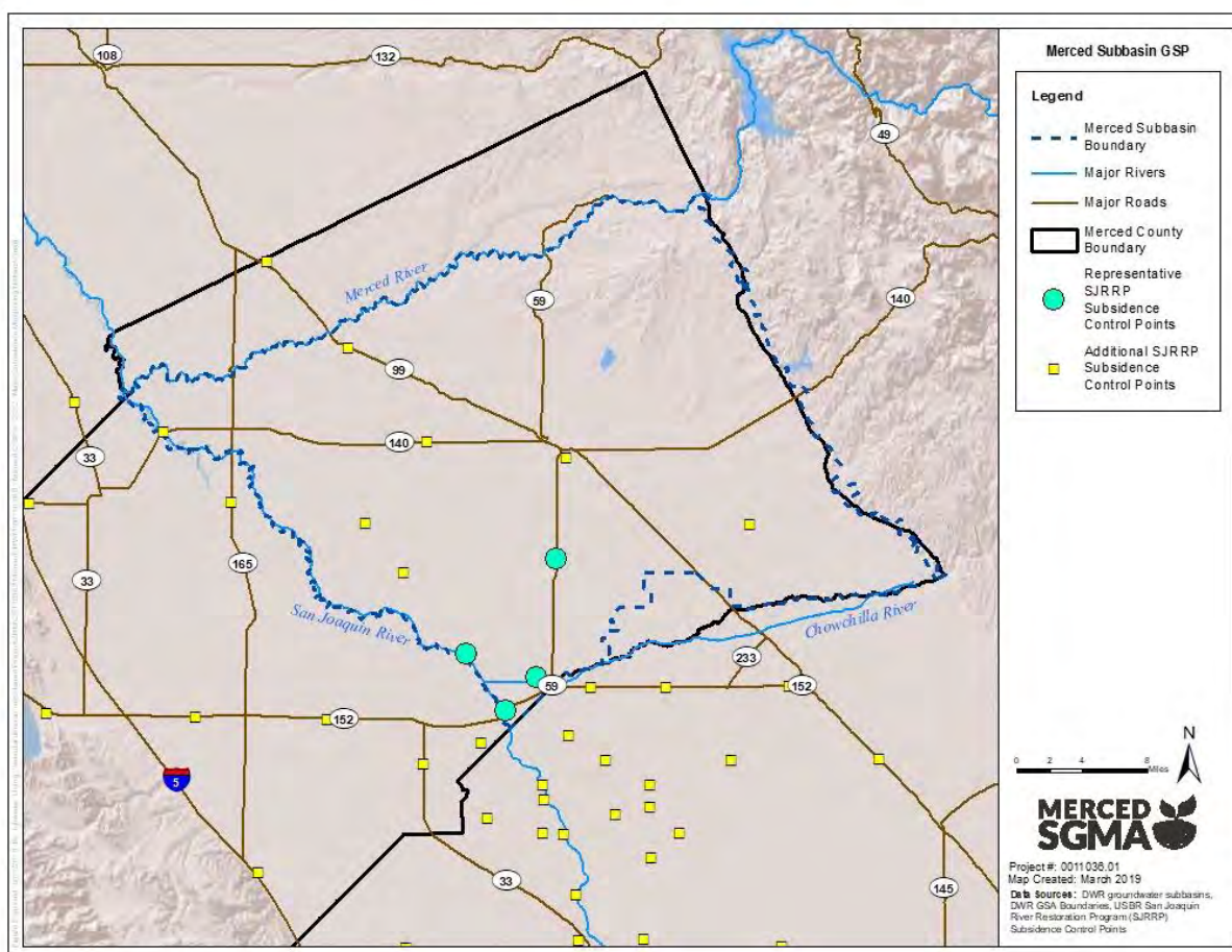
Figure 4-8: Merced Subbasin GSP Subsidence Monitoring Network Sites
