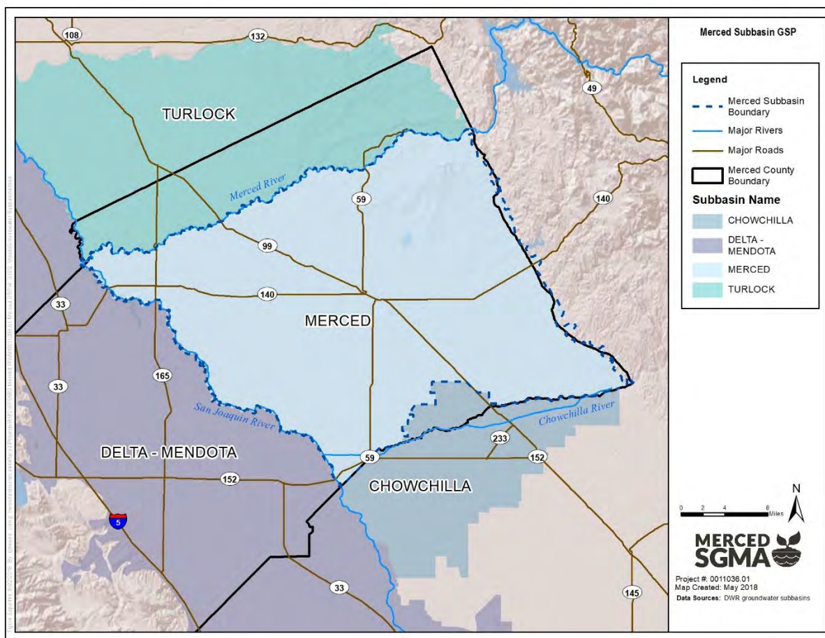
Figure 2-27: Neighboring Subbasins
