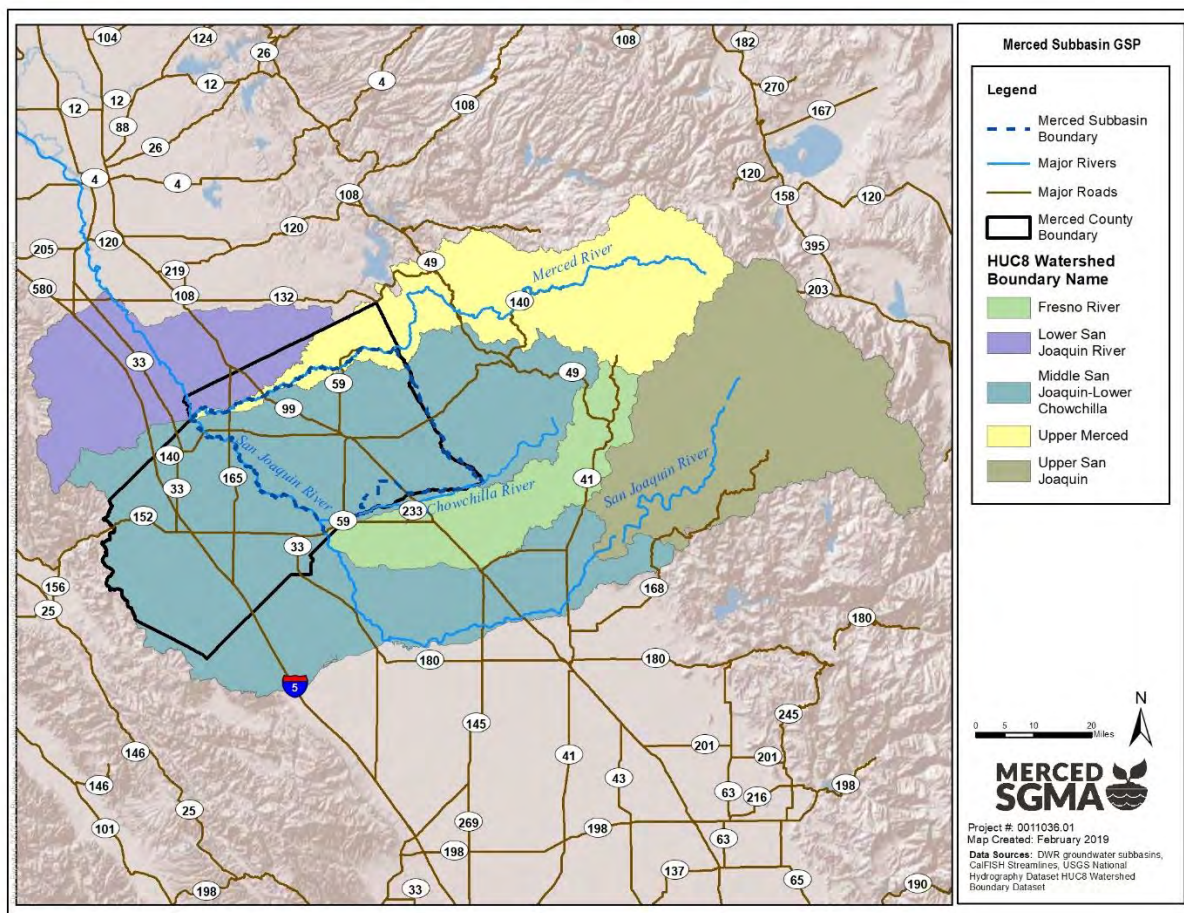
Figure 2-7: HUC8 Watershed Boundaries
