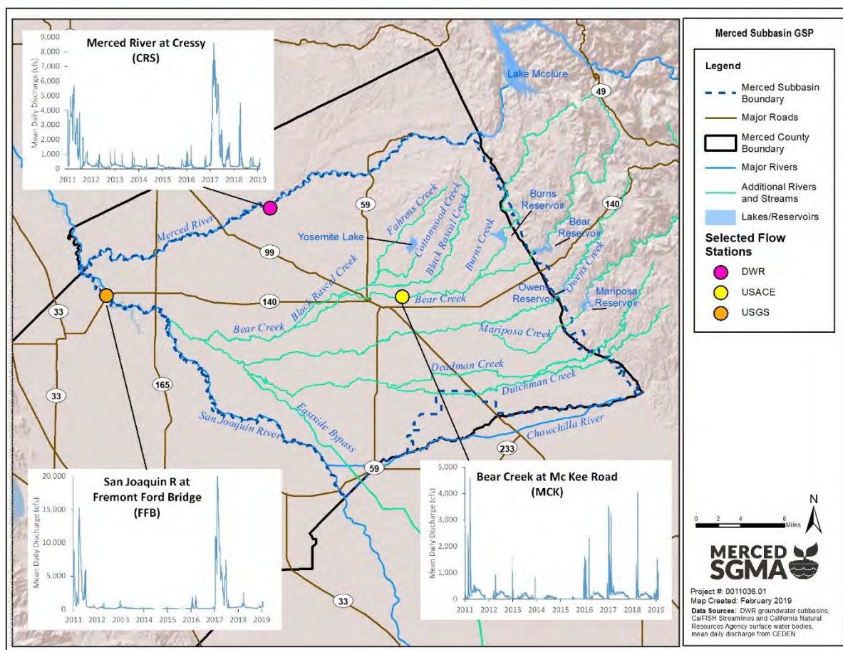
Figure 2-5: Surface Waters
