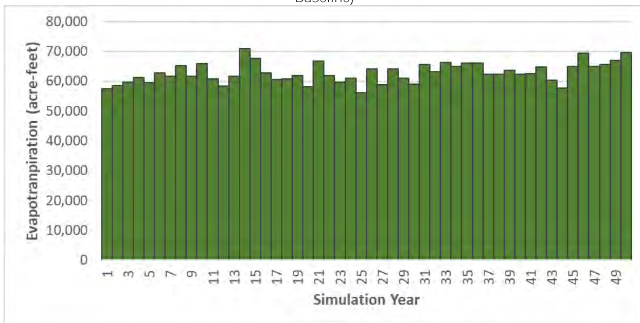
Figure 2-116: Simulated changes in Evapotranspiration due to Climate Change (Scenario minus Baseline)
