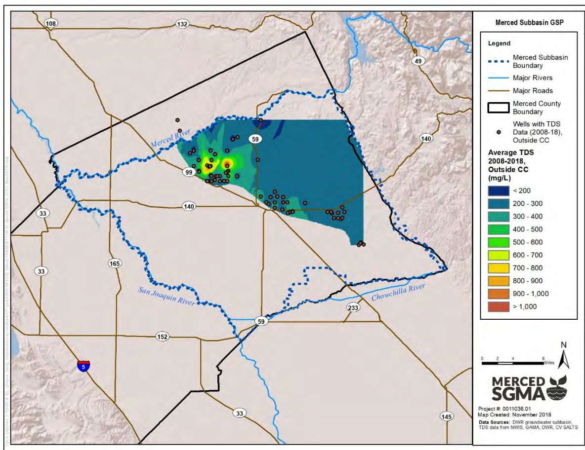
Figure 2-65: Average TDS Concentration 2008-2018, Outside Corcoran Clay
