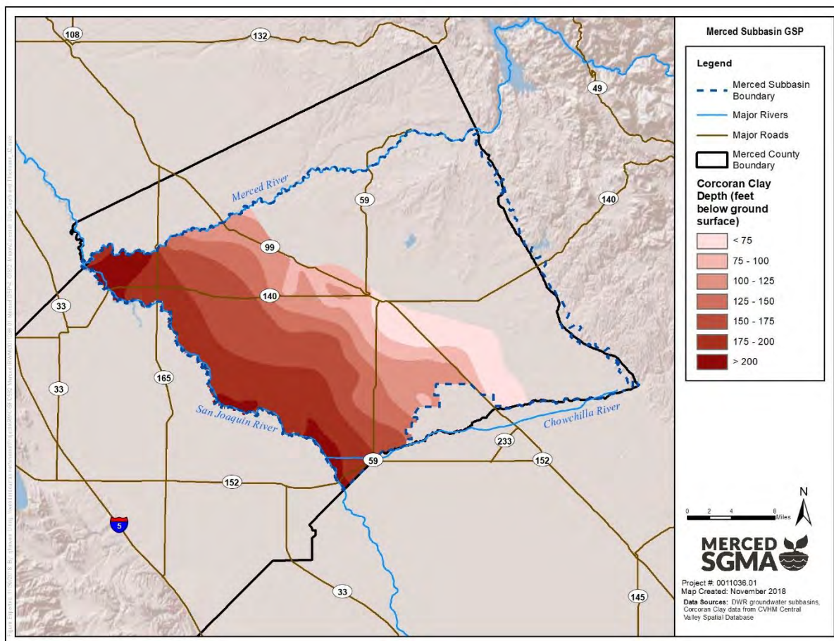
Figure 2-37: Corcoran Clay Depth Below Ground Surface
