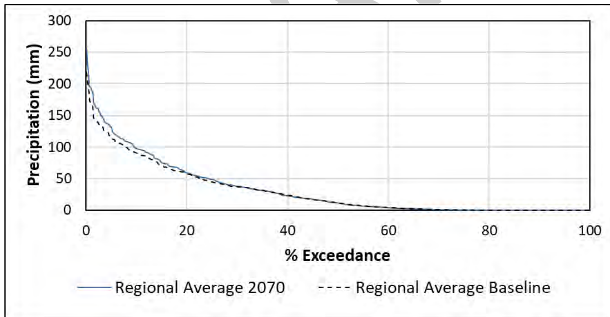
Figure 2-113: Perturbed Precipitation Exceedance Curve
