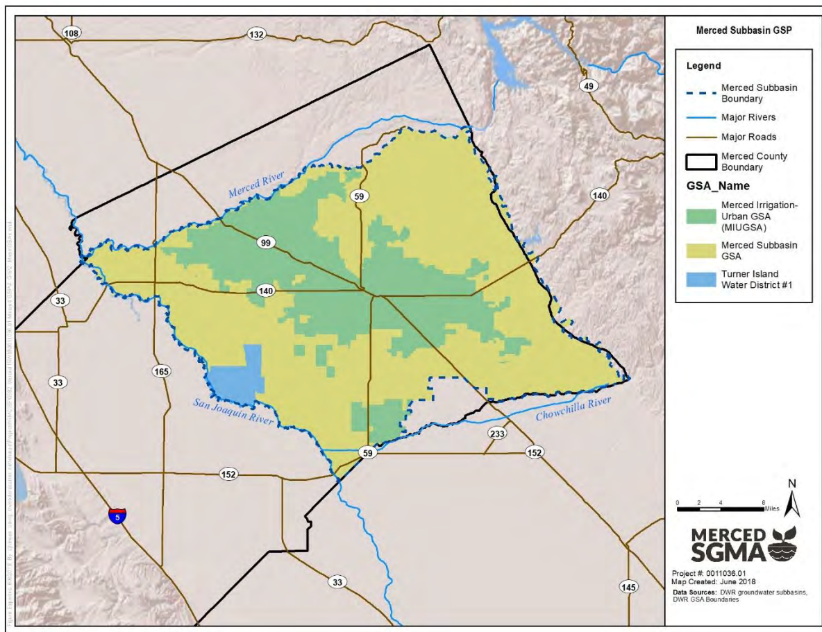
Figure 1-5: GSA Boundaries
