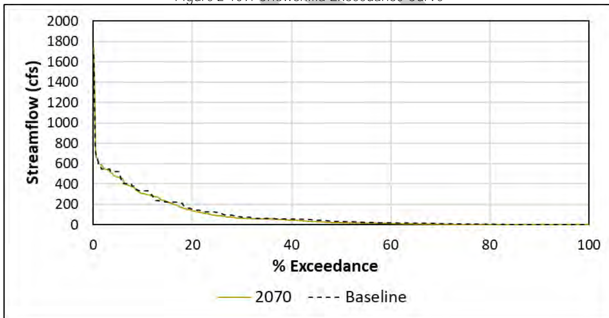
Figure 2-109: Chowchilla Exceedance Curve
