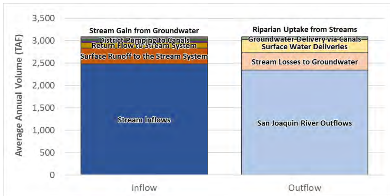
Figure 2-94: Current Conditions Average Annual Water Budget – Stream and Canal Systems, Merced Subbasin
