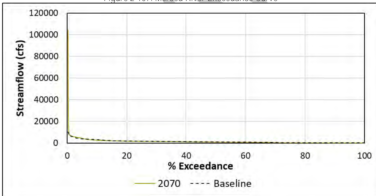
Figure 2-107: Merced River Exceedance Curve
