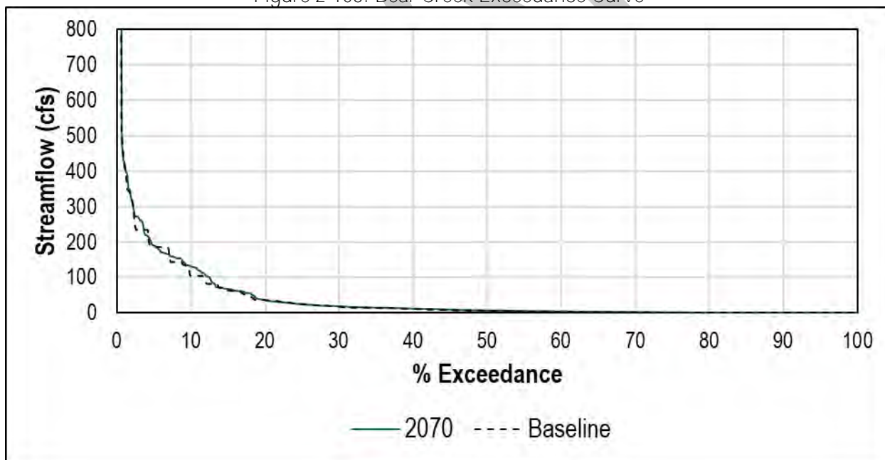
Figure 2-103: Bear Creek Exceedance Curve
