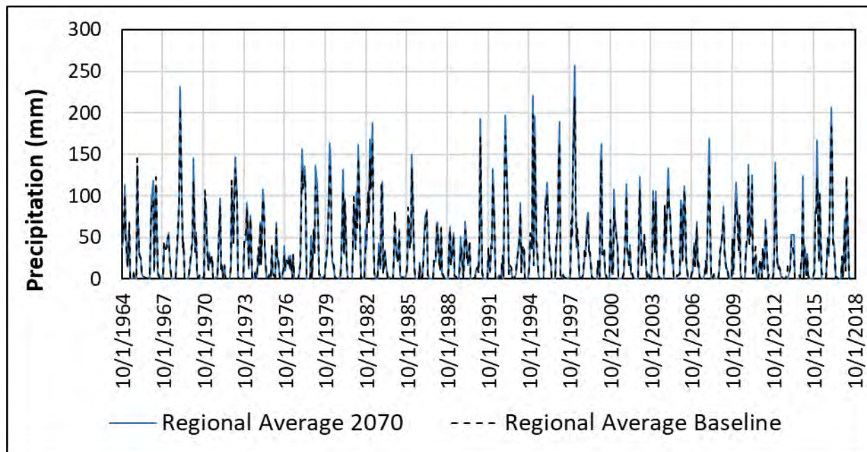
Figure 2-112: Perturbed Precipitation Under Climate Change
